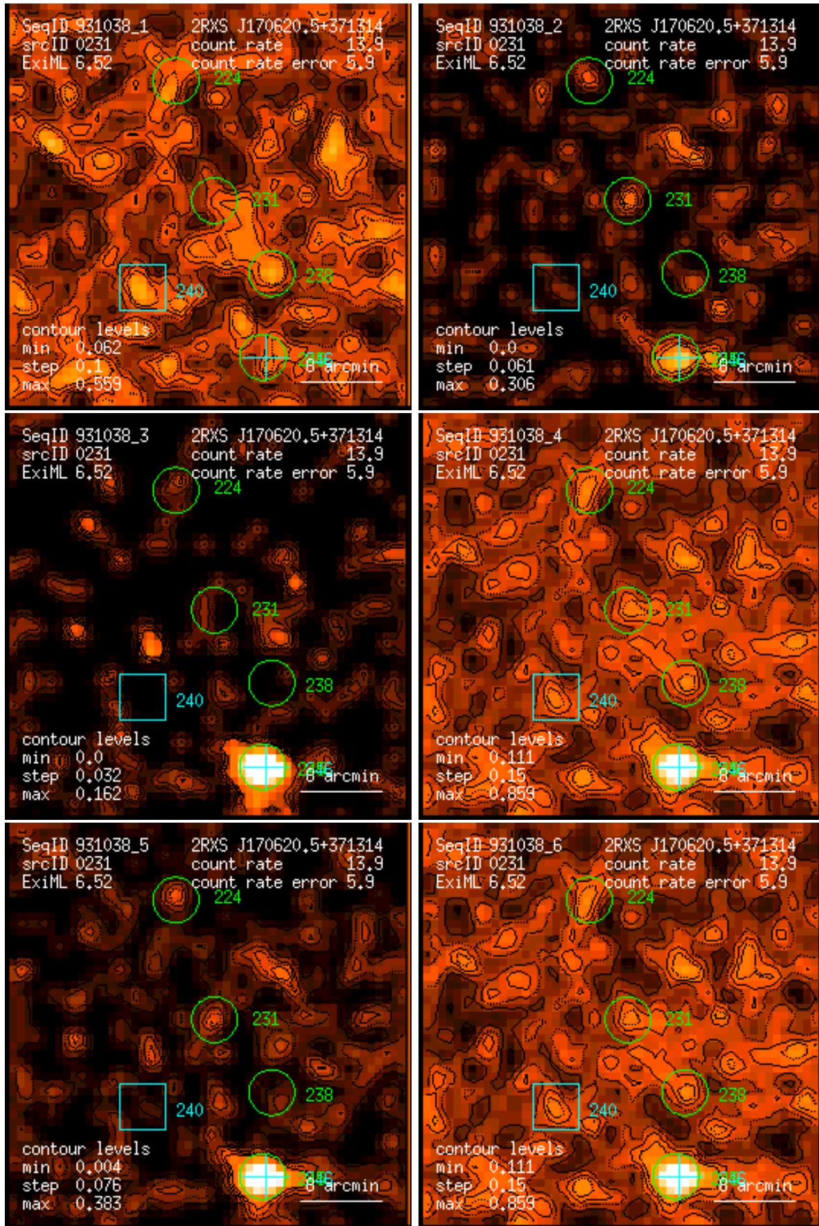
Figure 231: RASS 931038: detection 0231: band rate images, Gaussian filter: (1) PSPC channels 11 – 41, (2) 52 – 90, (3) 91 – 201, (4) 11 – 235, (5) 52 – 201, (6) 11 – 201. Broad band rates in counts/ks. Band rate contour levels in counts/ks/arcmin 2 .
