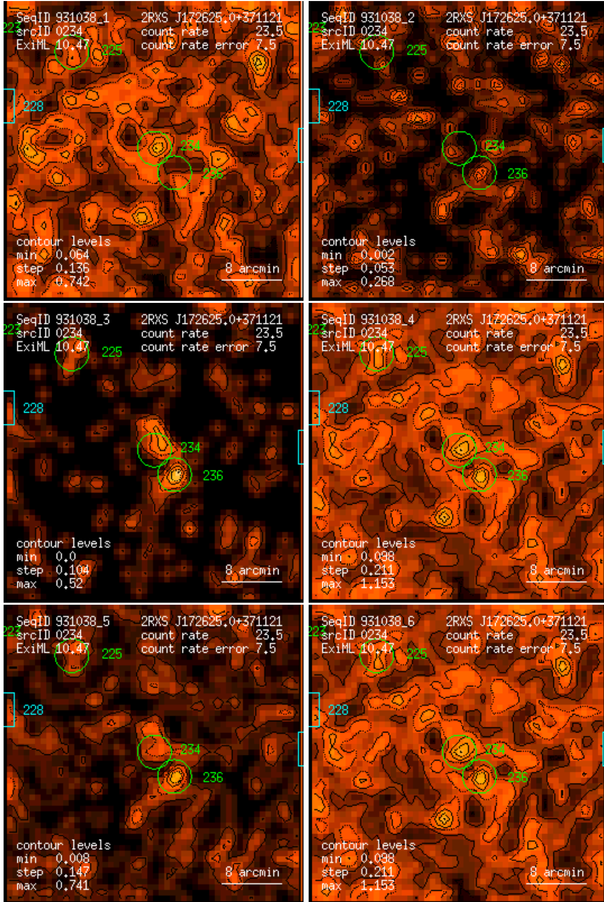
Figure 234: RASS 931038: detection 0234: band rate images, Gaussian filter: (1) PSPC channels 11 – 41, (2) 52 – 90, (3) 91 – 201, (4) 11 – 235, (5) 52 – 201, (6) 11 – 201. Broad band rates in counts/ks. Band rate contour levels in counts/ks/arcmin 2 .
