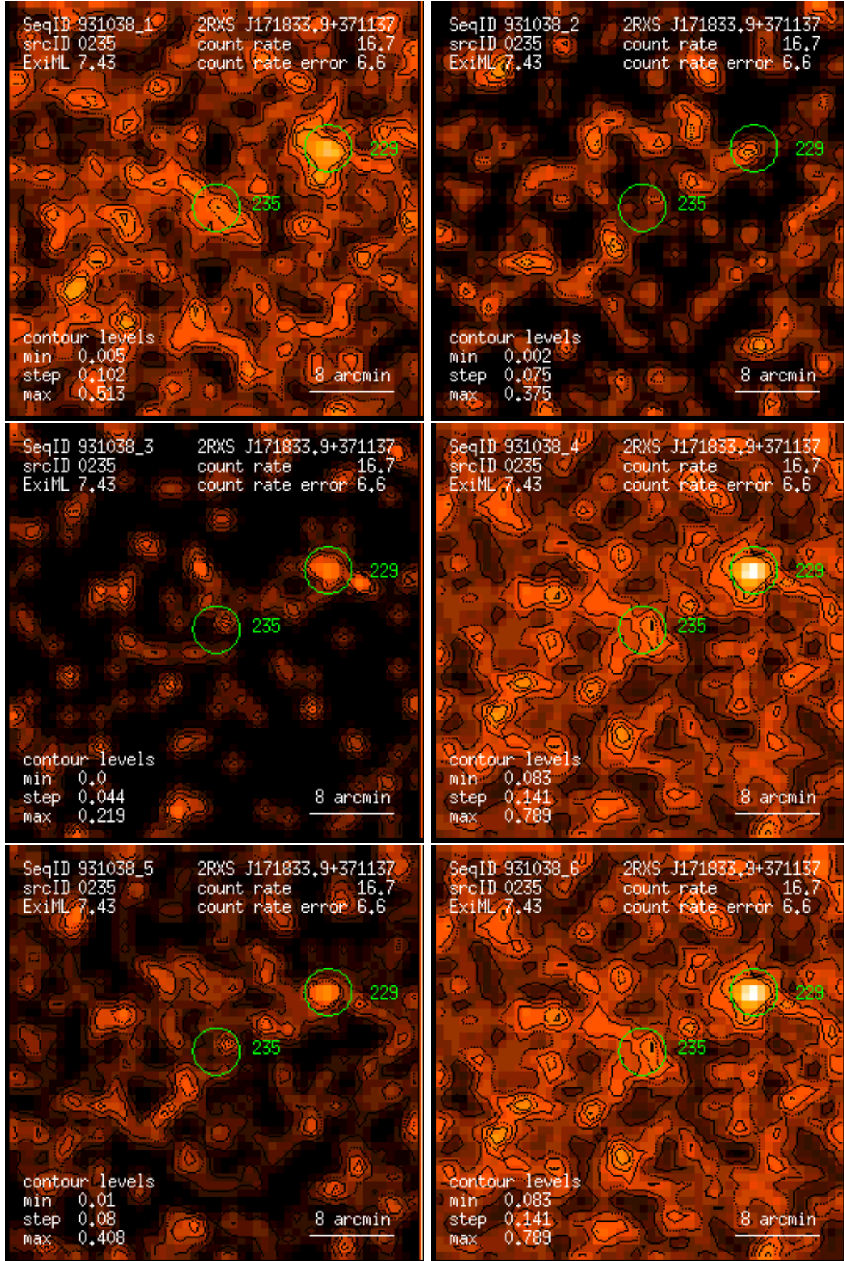
Figure 235: RASS 931038: detection 0235: band rate images, Gaussian filter: (1) PSPC channels 11 – 41, (2) 52 – 90, (3) 91 – 201, (4) 11 – 235, (5) 52 – 201, (6) 11 – 201. Broad band rates in counts/ks. Band rate contour levels in counts/ks/arcmin 2 .
