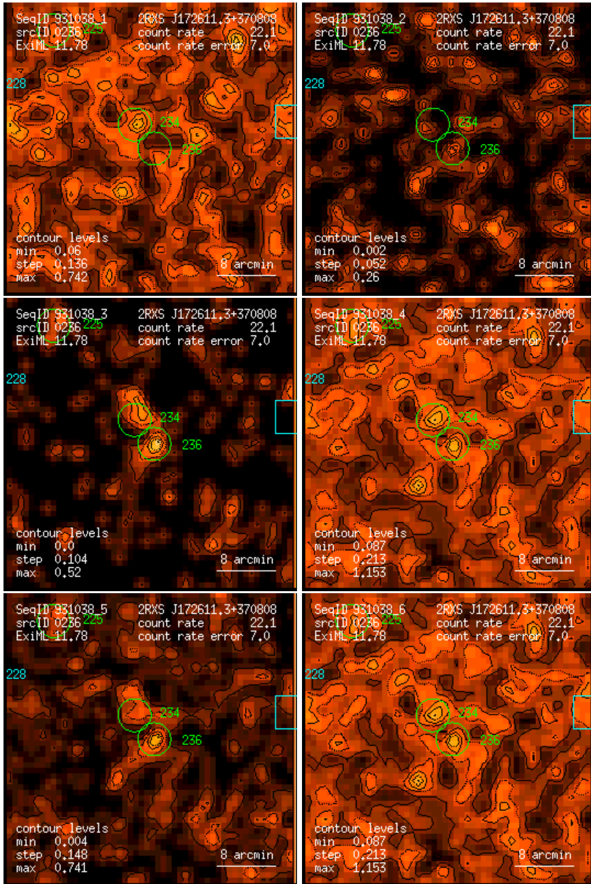
Figure 236: RASS 931038: detection 0236: band rate images, Gaussian filter: (1) PSPC channels 11 – 41, (2) 52 – 90, (3) 91 – 201, (4) 11 – 235, (5) 52 – 201, (6) 11 – 201. Broad band rates in counts/ks. Band rate contour levels in counts/ks/arcmin 2 .
