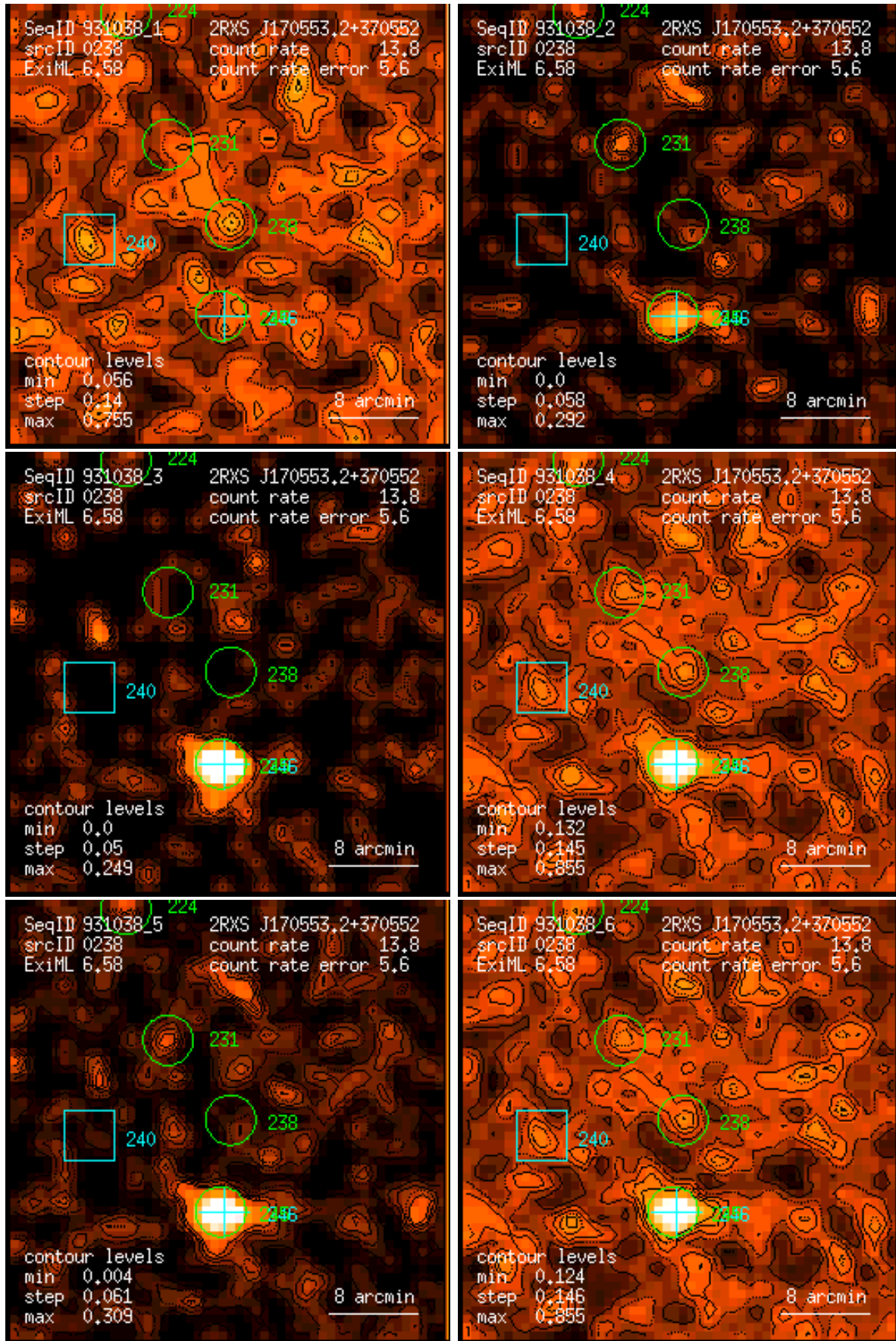
Figure 238: RASS 931038: detection 0238: band rate images, Gaussian filter: (1) PSPC channels 11 – 41, (2) 52 – 90, (3) 91 – 201, (4) 11 – 235, (5) 52 – 201, (6) 11 – 201. Broad band rates in counts/ks. Band rate contour levels in counts/ks/arcmin 2 .
