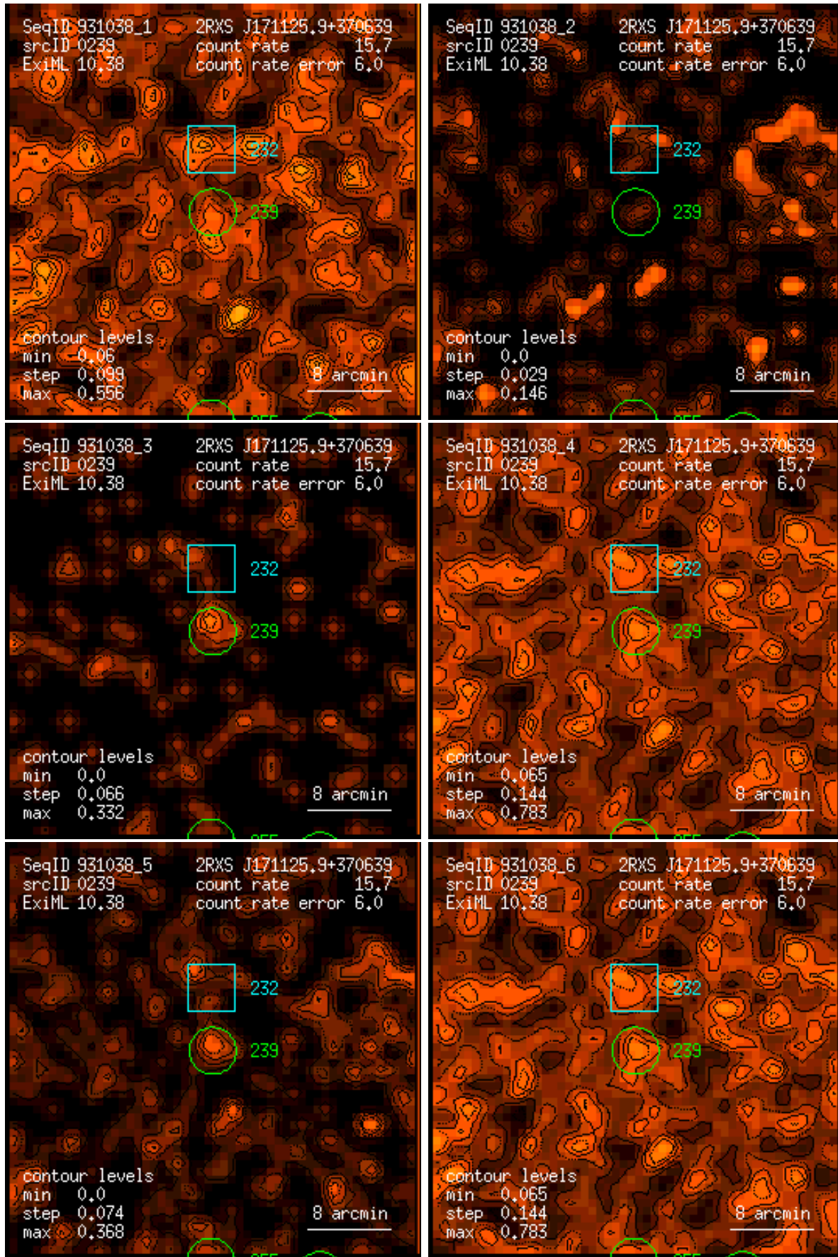
Figure 239: RASS 931038: detection 0239: band rate images, Gaussian filter: (1) PSPC channels 11 – 41, (2) 52 – 90, (3) 91 – 201, (4) 11 – 235, (5) 52 – 201, (6) 11 – 201. Broad band rates in counts/ks. Band rate contour levels in counts/ks/arcmin 2 .
