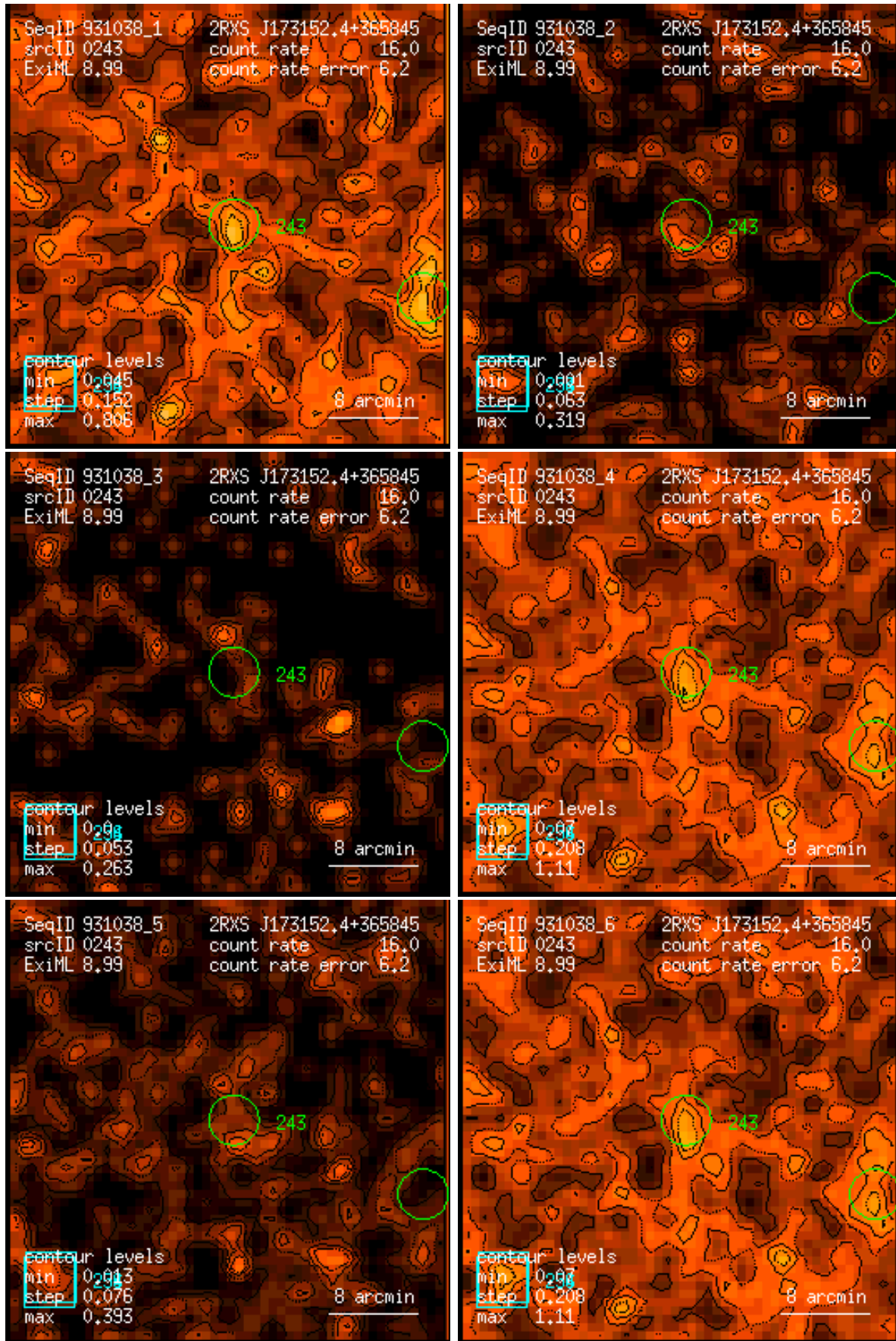
Figure 243: RASS 931038: detection 0243: band rate images, Gaussian filter: (1) PSPC channels 11 – 41, (2) 52 – 90, (3) 91 – 201, (4) 11 – 235, (5) 52 – 201, (6) 11 – 201. Broad band rates in counts/ks. Band rate contour levels in counts/ks/arcmin 2 .
