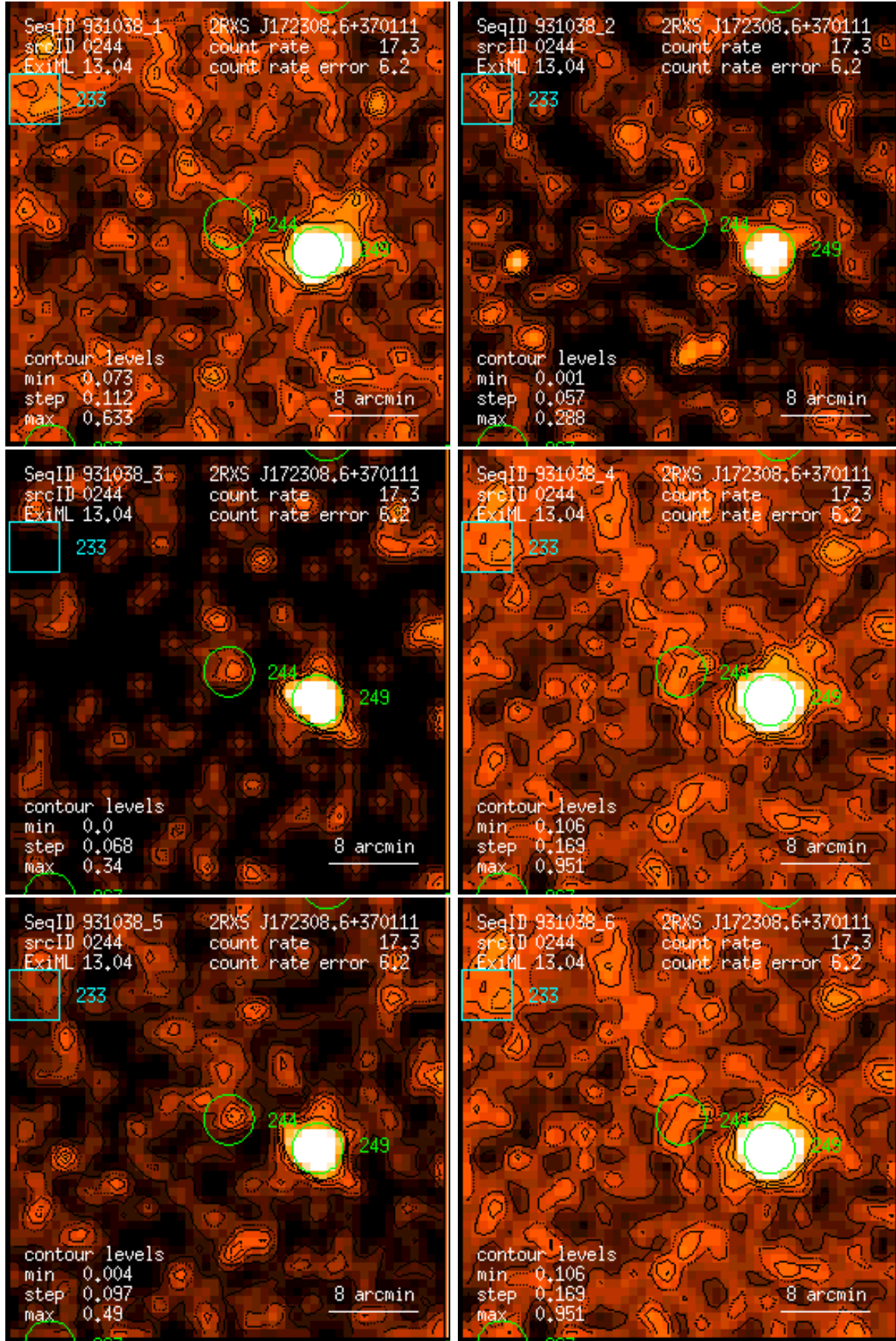
Figure 244: RASS 931038: detection 0244: band rate images, Gaussian filter: (1) PSPC channels 11 – 41, (2) 52 – 90, (3) 91 – 201, (4) 11 – 235, (5) 52 – 201, (6) 11 – 201. Broad band rates in counts/ks. Band rate contour levels in counts/ks/arcmin 2 .
