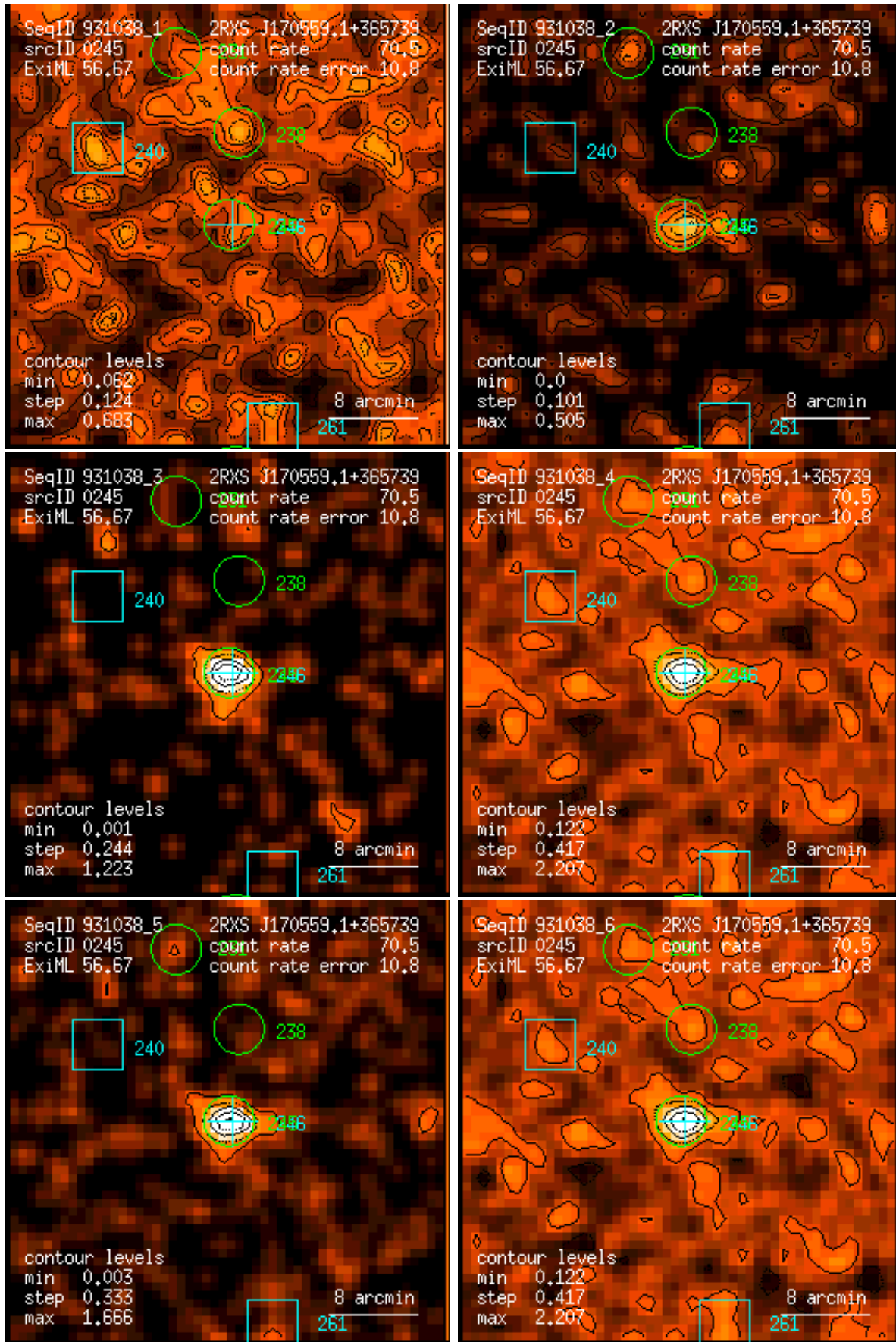
Figure 245: RASS 931038: detection 0245: band rate images, Gaussian filter: (1) PSPC channels 11 – 41, (2) 52 – 90, (3) 91 – 201, (4) 11 – 235, (5) 52 – 201, (6) 11 – 201. Broad band rates in counts/ks. Band rate contour levels in counts/ks/arcmin 2 .
