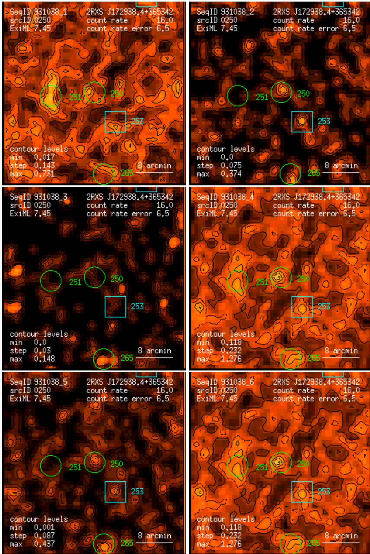
Figure 250: RASS 931038: detection 0250: band rate images, Gaussian filter: (1) PSPC channels 11 – 41, (2) 52 – 90, (3) 91 – 201, (4) 11 – 235, (5) 52 – 201, (6) 11 – 201. Broad band rates in counts/ks. Band rate contour levels in counts/ks/arcmin 2 .
