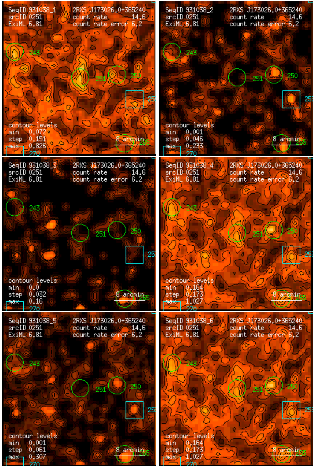
Figure 251: RASS 931038: detection 0251: band rate images, Gaussian filter: (1) PSPC channels 11 – 41, (2) 52 – 90, (3) 91 – 201, (4) 11 – 235, (5) 52 – 201, (6) 11 – 201. Broad band rates in counts/ks. Band rate contour levels in counts/ks/arcmin 2 .
