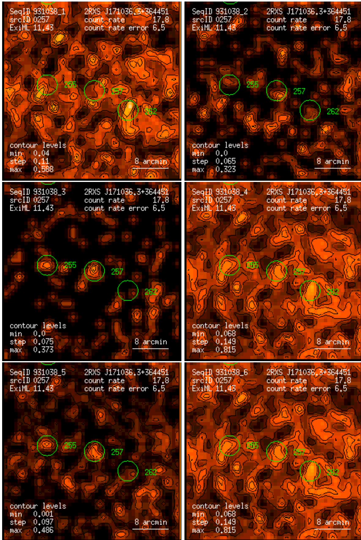
Figure 257: RASS 931038: detection 0257: band rate images, Gaussian filter: (1) PSPC channels 11 – 41, (2) 52 – 90, (3) 91 – 201, (4) 11 – 235, (5) 52 – 201, (6) 11 – 201. Broad band rates in counts/ks. Band rate contour levels in counts/ks/arcmin 2 .
