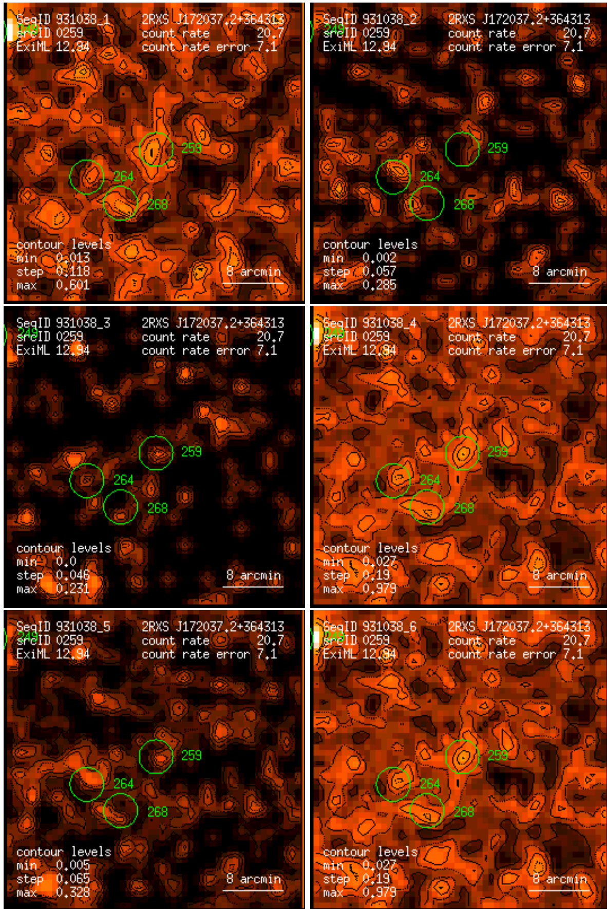
Figure 259: RASS 931038: detection 0259: band rate images, Gaussian filter: (1) PSPC channels 11 – 41, (2) 52 – 90, (3) 91 – 201, (4) 11 – 235, (5) 52 – 201, (6) 11 – 201. Broad band rates in counts/ks. Band rate contour levels in counts/ks/arcmin 2 .
