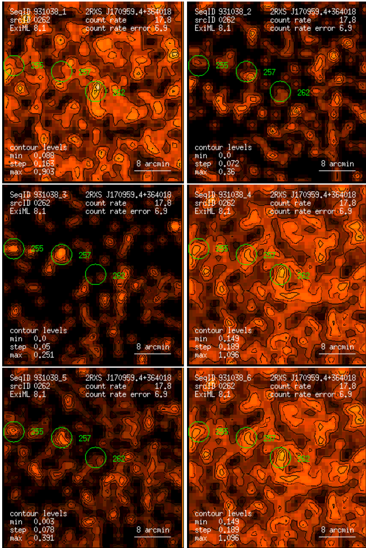
Figure 262: RASS 931038: detection 0262: band rate images, Gaussian filter: (1) PSPC channels 11 – 41, (2) 52 – 90, (3) 91 – 201, (4) 11 – 235, (5) 52 – 201, (6) 11 – 201. Broad band rates in counts/ks. Band rate contour levels in counts/ks/arcmin 2 .
