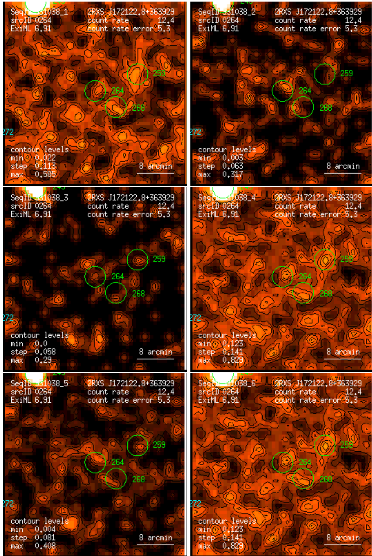
Figure 264: RASS 931038: detection 0264: band rate images, Gaussian filter: (1) PSPC channels 11 – 41, (2) 52 – 90, (3) 91 – 201, (4) 11 – 235, (5) 52 – 201, (6) 11 – 201. Broad band rates in counts/ks. Band rate contour levels in counts/ks/arcmin 2 .
