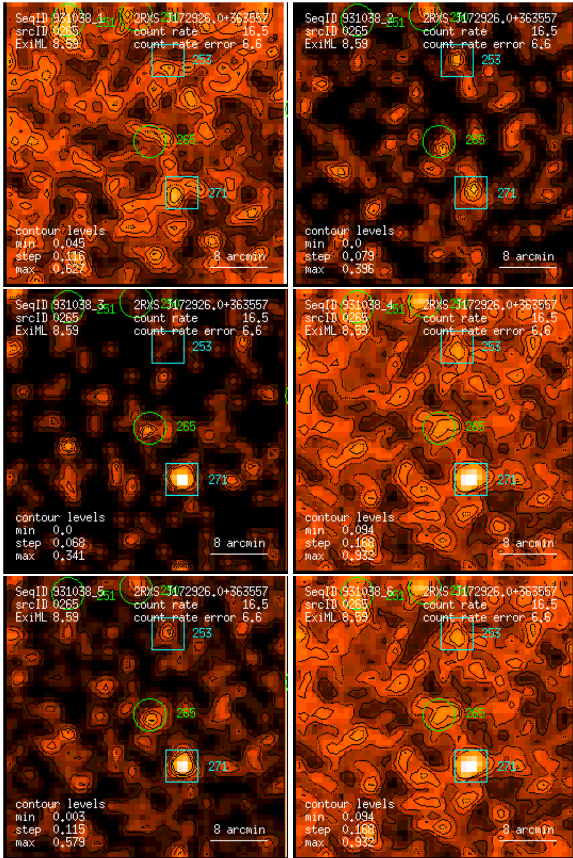
Figure 265: RASS 931038: detection 0265: band rate images, Gaussian filter: (1) PSPC channels 11 – 41, (2) 52 – 90, (3) 91 – 201, (4) 11 – 235, (5) 52 – 201, (6) 11 – 201. Broad band rates in counts/ks. Band rate contour levels in counts/ks/arcmin 2 .
