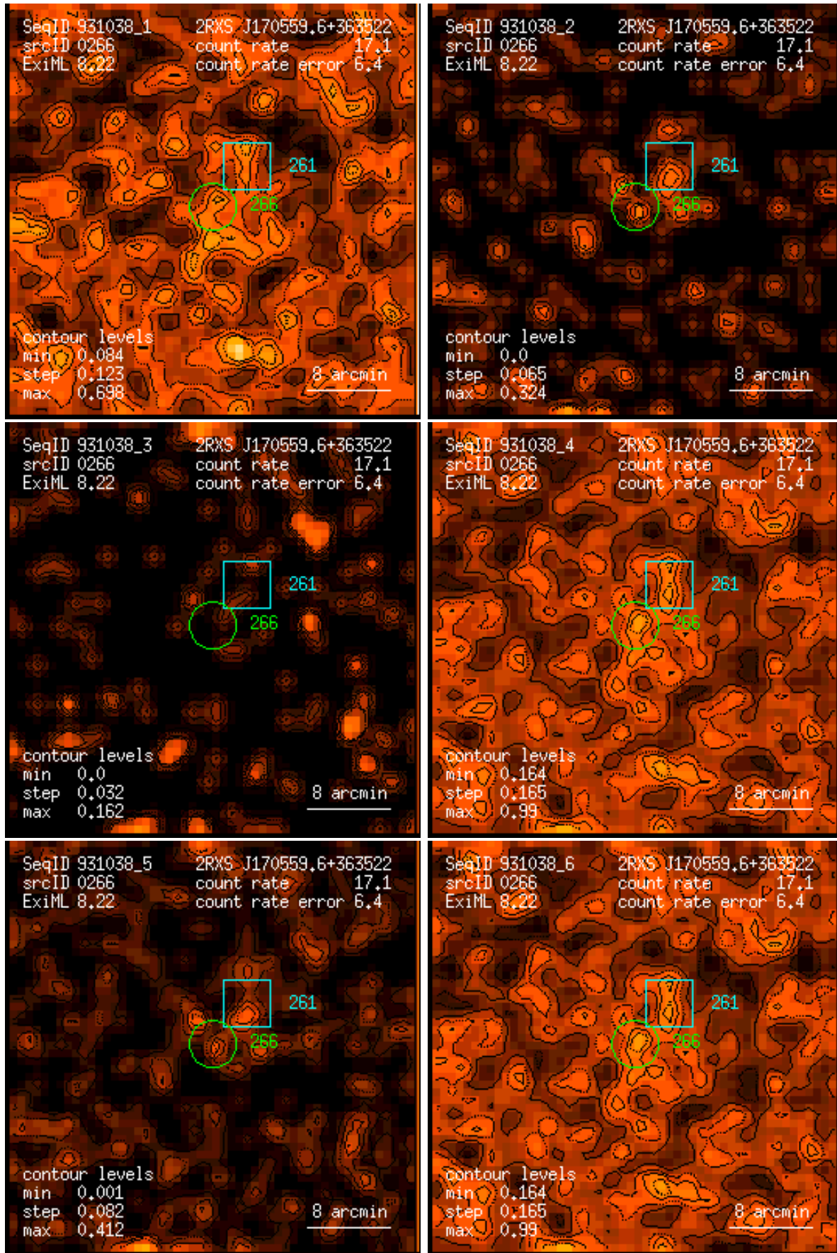
Figure 266: RASS 931038: detection 0266: band rate images, Gaussian filter: (1) PSPC channels 11 – 41, (2) 52 – 90, (3) 91 – 201, (4) 11 – 235, (5) 52 – 201, (6) 11 – 201. Broad band rates in counts/ks. Band rate contour levels in counts/ks/arcmin 2 .
