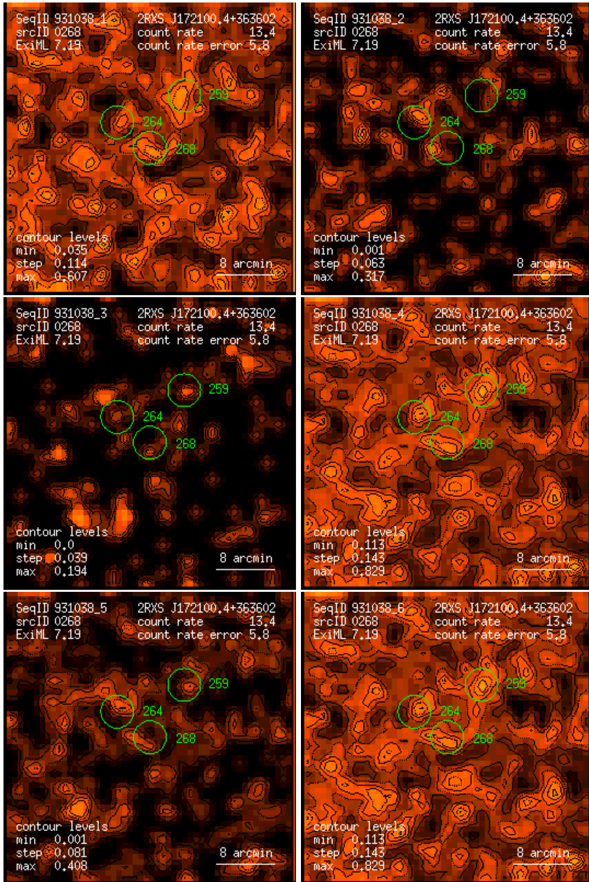
Figure 268: RASS 931038: detection 0268: band rate images, Gaussian filter: (1) PSPC channels 11 – 41, (2) 52 – 90, (3) 91 – 201, (4) 11 – 235, (5) 52 – 201, (6) 11 – 201. Broad band rates in counts/ks. Band rate contour levels in counts/ks/arcmin 2 .
