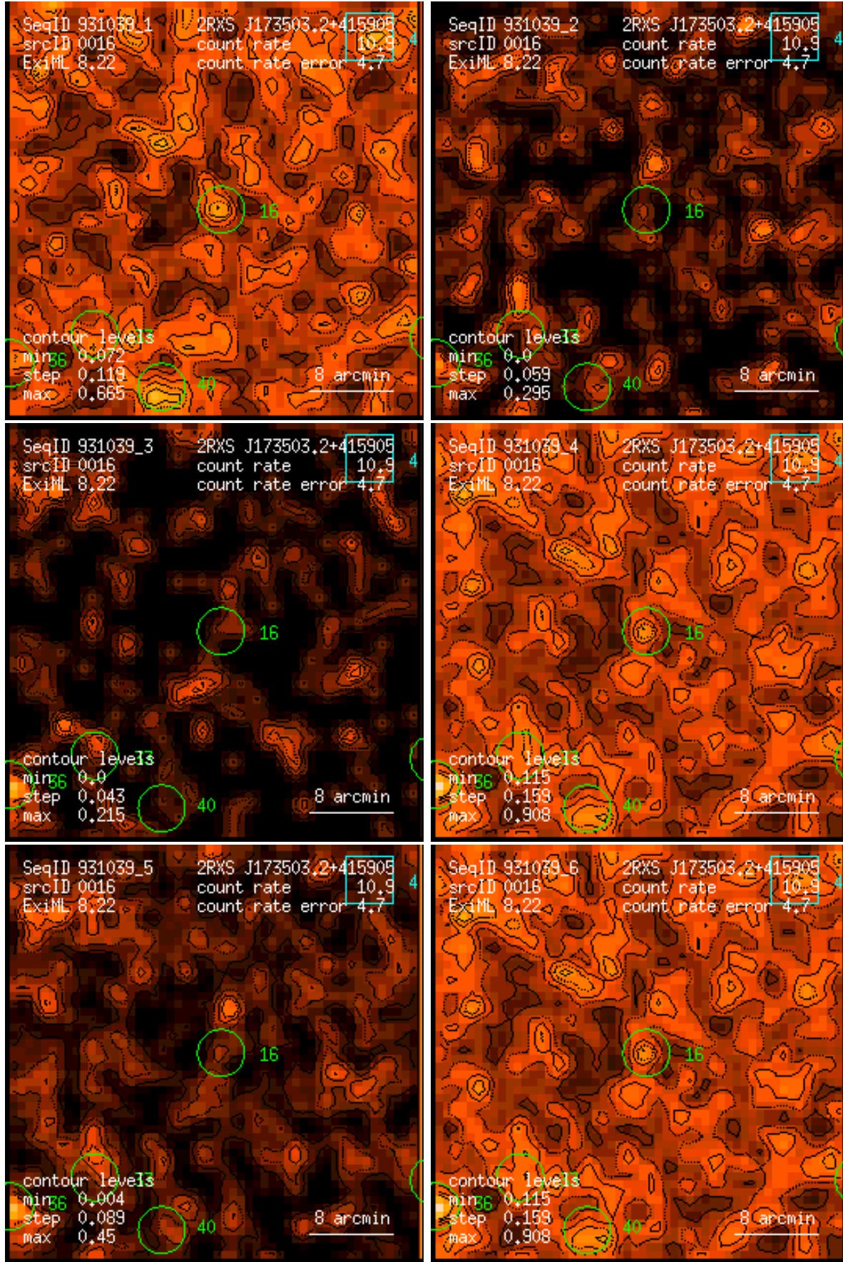
Figure 16: RASS 931039: detection 0016: band rate images, Gaussian filter: (1) PSPC channels 11 – 41, (2) 52 – 90, (3) 91 – 201, (4) 11 – 235, (5) 52 – 201, (6) 11 – 201. Broad band rates in counts/ks. Band rate contour levels in counts/ks/arcmin 2 .
