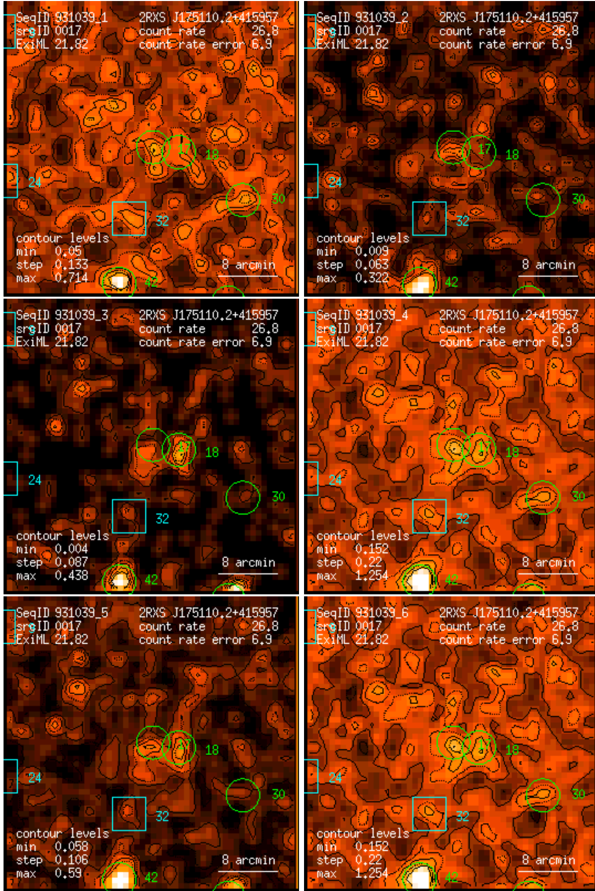
Figure 17: RASS 931039: detection 0017: band rate images, Gaussian filter: (1) PSPC channels 11 – 41, (2) 52 – 90, (3) 91 – 201, (4) 11 – 235, (5) 52 – 201, (6) 11 – 201. Broad band rates in counts/ks. Band rate contour levels in counts/ks/arcmin 2 .
