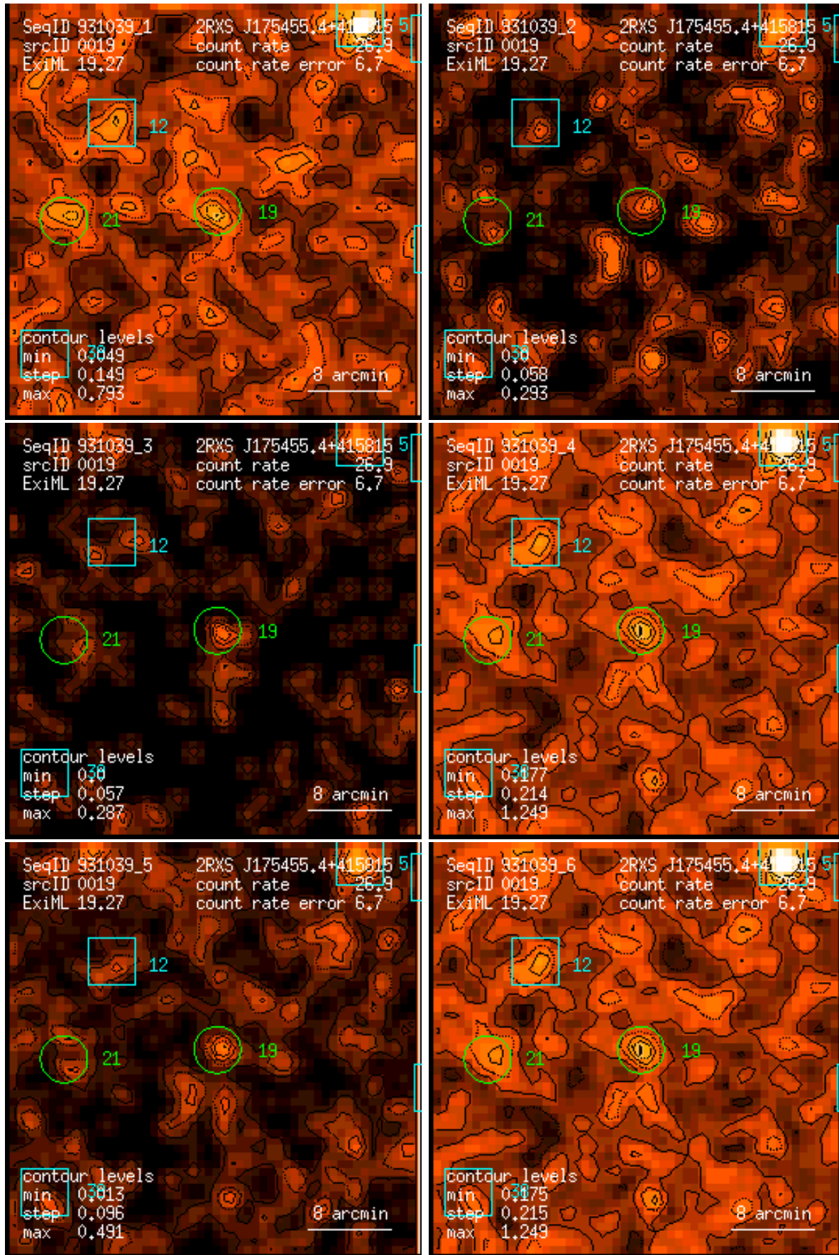
Figure 19: RASS 931039: detection 0019: band rate images, Gaussian filter: (1) PSPC channels 11 – 41, (2) 52 – 90, (3) 91 – 201, (4) 11 – 235, (5) 52 – 201, (6) 11 – 201. Broad band rates in counts/ks. Band rate contour levels in counts/ks/arcmin 2 .
