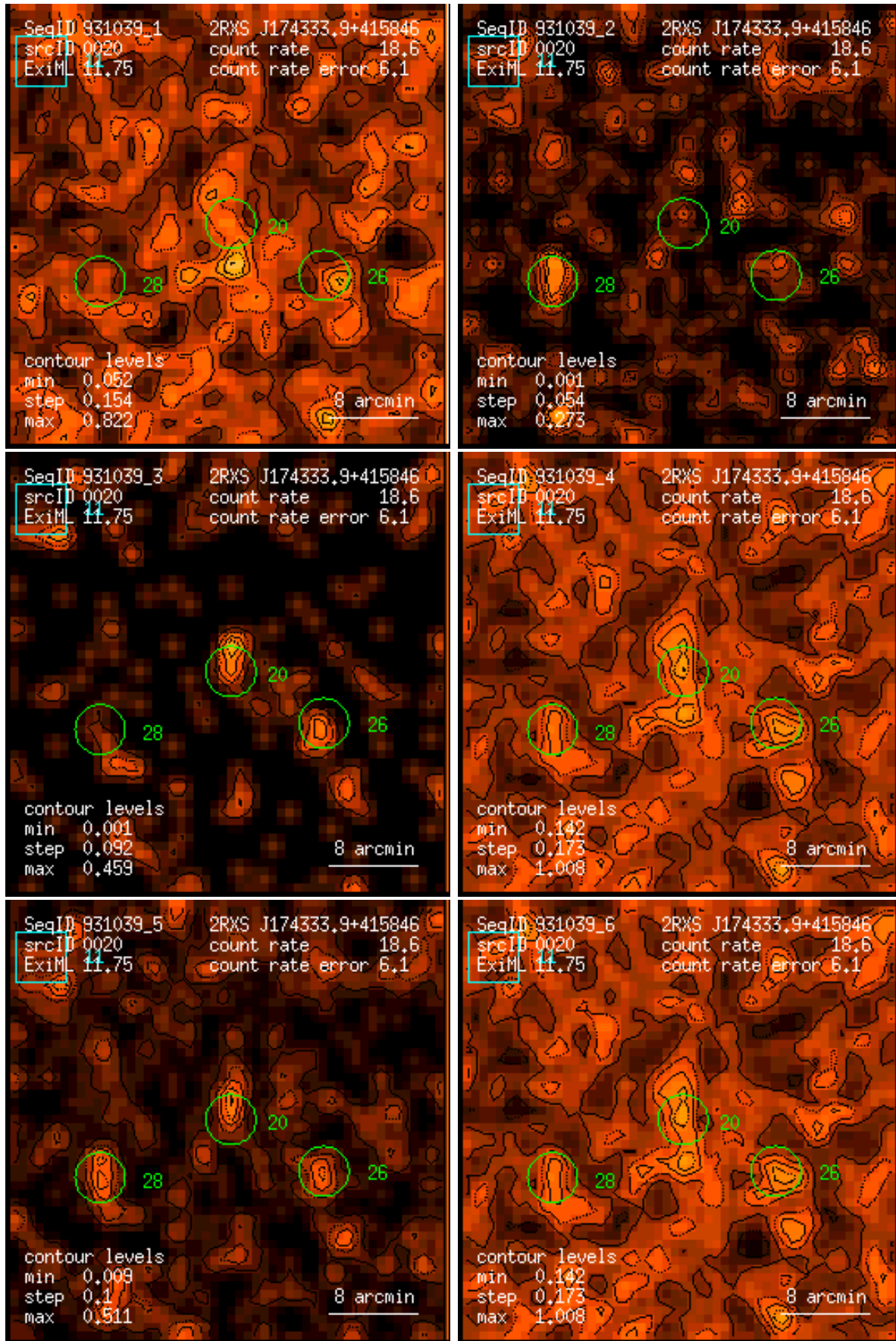
Figure 20: RASS 931039: detection 0020: band rate images, Gaussian filter: (1) PSPC channels 11 – 41, (2) 52 – 90, (3) 91 – 201, (4) 11 – 235, (5) 52 – 201, (6) 11 – 201. Broad band rates in counts/ks. Band rate contour levels in counts/ks/arcmin 2 .
