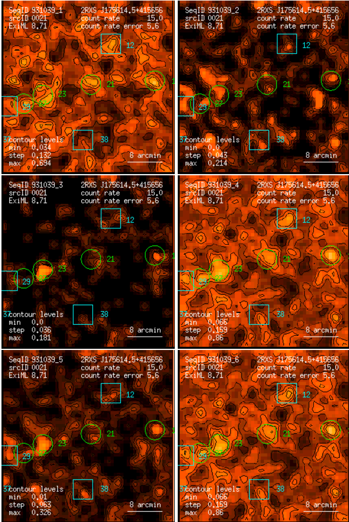
Figure 21: RASS 931039: detection 0021: band rate images, Gaussian filter: (1) PSPC channels 11 – 41, (2) 52 – 90, (3) 91 – 201, (4) 11 – 235, (5) 52 – 201, (6) 11 – 201. Broad band rates in counts/ks. Band rate contour levels in counts/ks/arcmin 2 .
