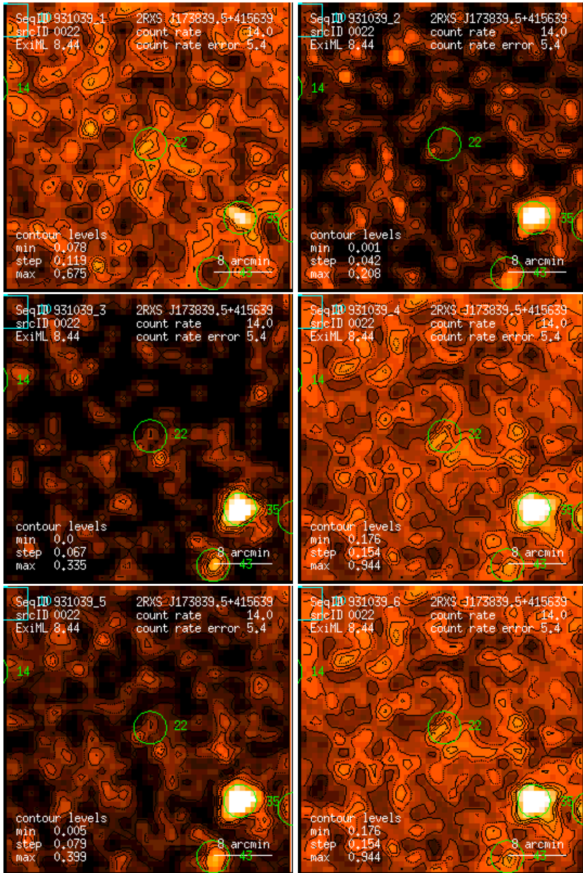
Figure 22: RASS 931039: detection 0022: band rate images, Gaussian filter: (1) PSPC channels 11 – 41, (2) 52 – 90, (3) 91 – 201, (4) 11 – 235, (5) 52 – 201, (6) 11 – 201. Broad band rates in counts/ks. Band rate contour levels in counts/ks/arcmin 2 .
