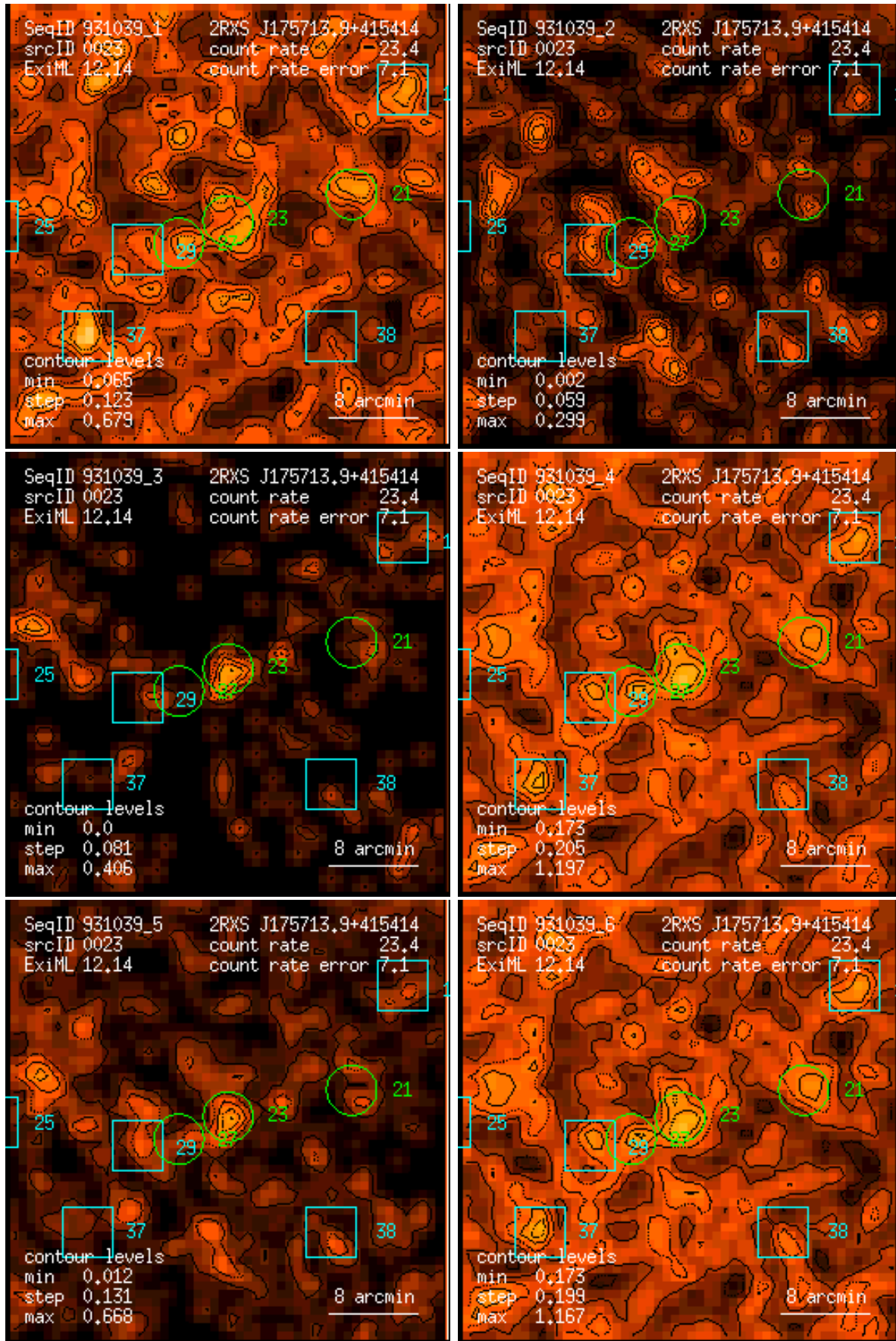
Figure 23: RASS 931039: detection 0023: band rate images, Gaussian filter: (1) PSPC channels 11 – 41, (2) 52 – 90, (3) 91 – 201, (4) 11 – 235, (5) 52 – 201, (6) 11 – 201. Broad band rates in counts/ks. Band rate contour levels in counts/ks/arcmin 2 .
