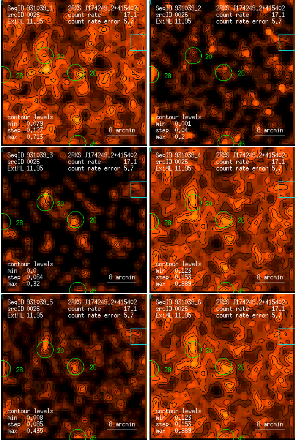
Figure 26: RASS 931039: detection 0026: band rate images, Gaussian filter: (1) PSPC channels 11 – 41, (2) 52 – 90, (3) 91 – 201, (4) 11 – 235, (5) 52 – 201, (6) 11 – 201. Broad band rates in counts/ks. Band rate contour levels in counts/ks/arcmin 2 .
