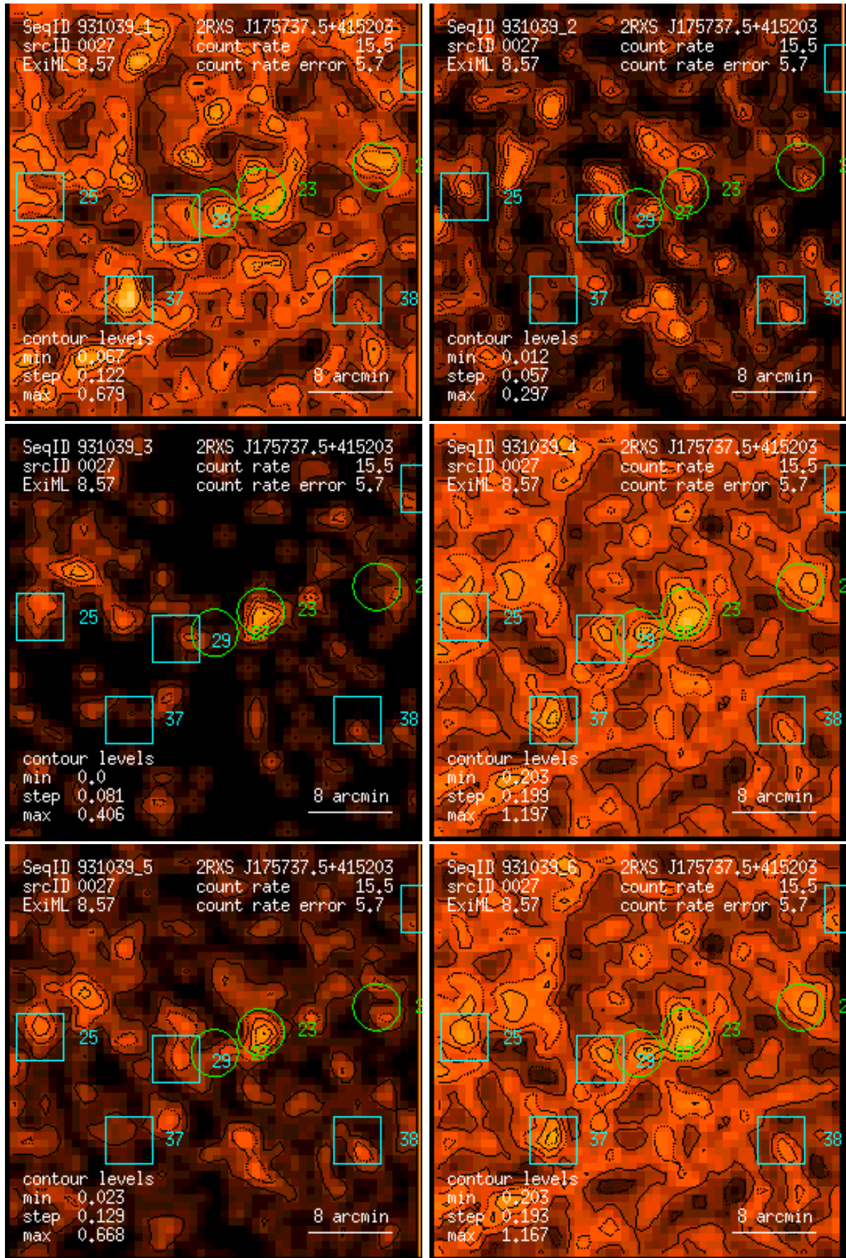
Figure 27: RASS 931039: detection 0027: band rate images, Gaussian filter: (1) PSPC channels 11 – 41, (2) 52 – 90, (3) 91 – 201, (4) 11 – 235, (5) 52 – 201, (6) 11 – 201. Broad band rates in counts/ks. Band rate contour levels in counts/ks/arcmin 2 .
