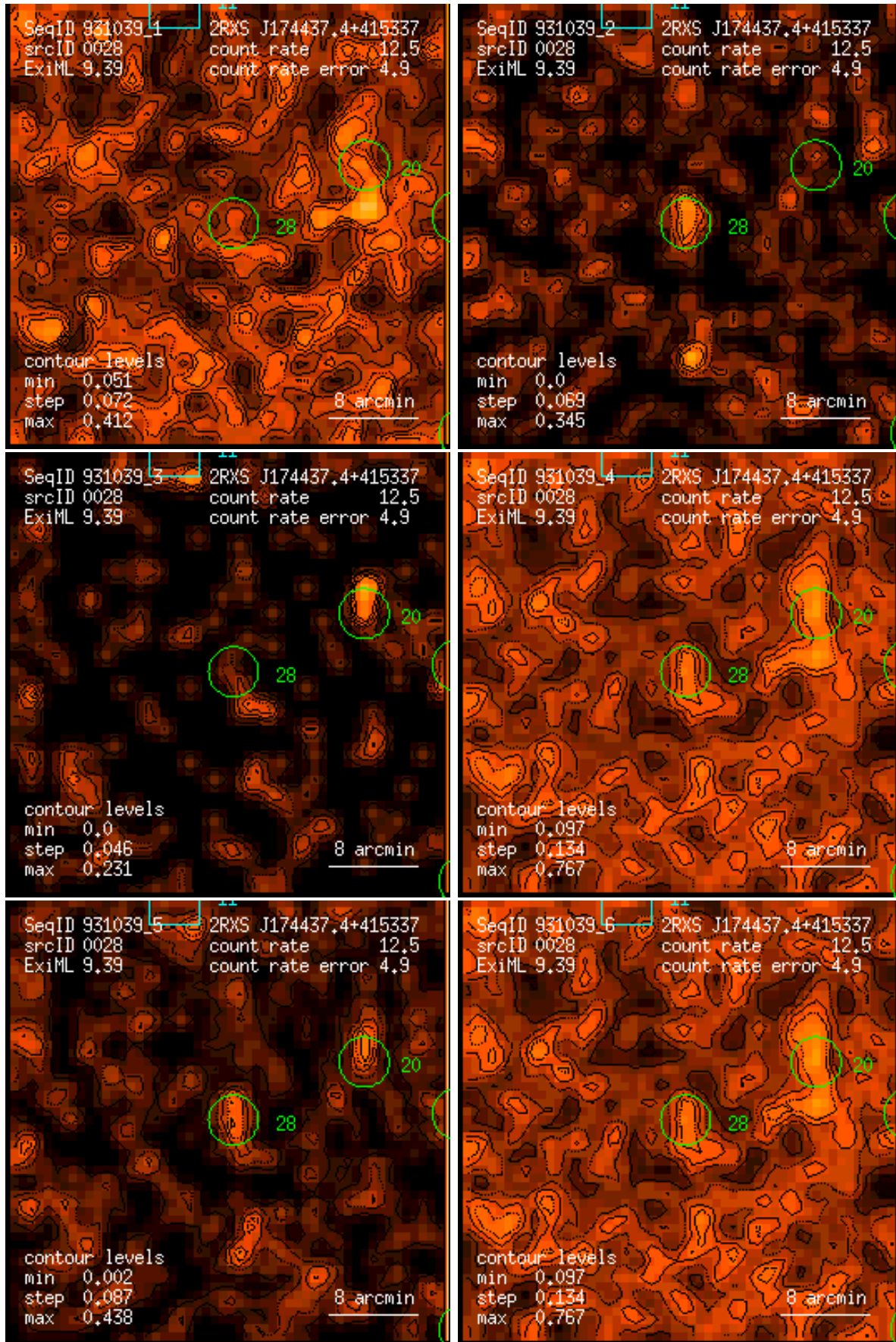
Figure 28: RASS 931039: detection 0028: band rate images, Gaussian filter: (1) PSPC channels 11 – 41, (2) 52 – 90, (3) 91 – 201, (4) 11 – 235, (5) 52 – 201, (6) 11 – 201. Broad band rates in counts/ks. Band rate contour levels in counts/ks/arcmin 2 .
