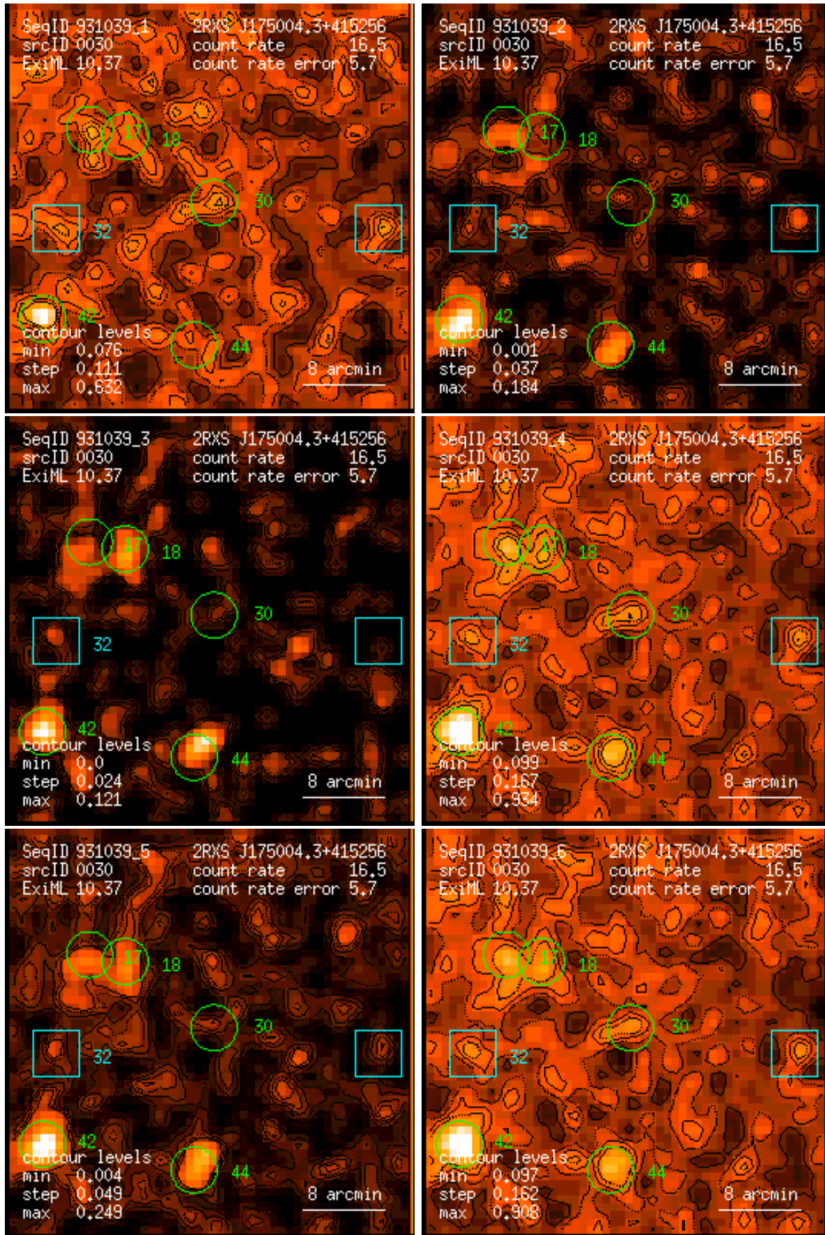
Figure 30: RASS 931039: detection 0030: band rate images, Gaussian filter: (1) PSPC channels 11 – 41, (2) 52 – 90, (3) 91 – 201, (4) 11 – 235, (5) 52 – 201, (6) 11 – 201. Broad band rates in counts/ks. Band rate contour levels in counts/ks/arcmin 2 .
