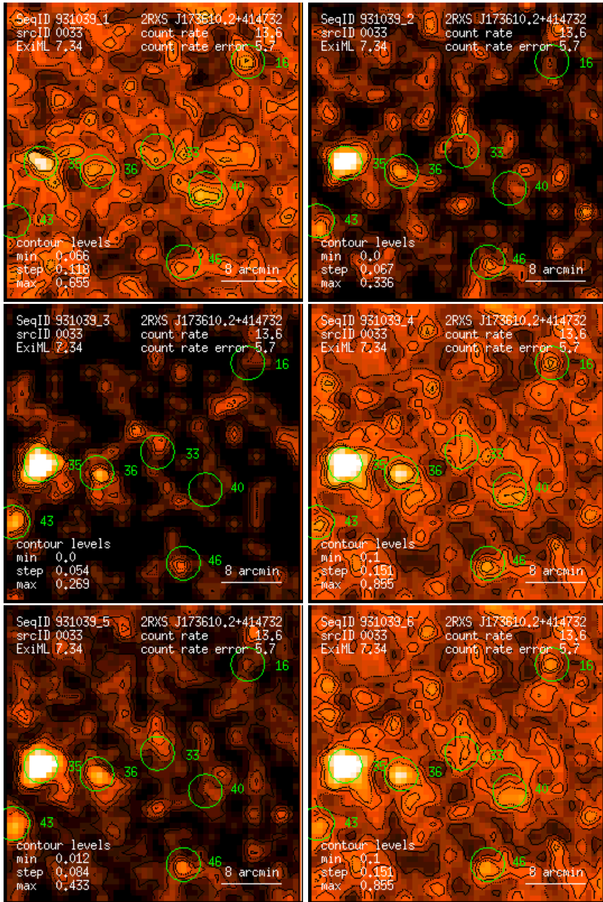
Figure 33: RASS 931039: detection 0033: band rate images, Gaussian filter: (1) PSPC channels 11 – 41, (2) 52 – 90, (3) 91 – 201, (4) 11 – 235, (5) 52 – 201, (6) 11 – 201. Broad band rates in counts/ks. Band rate contour levels in counts/ks/arcmin 2 .
