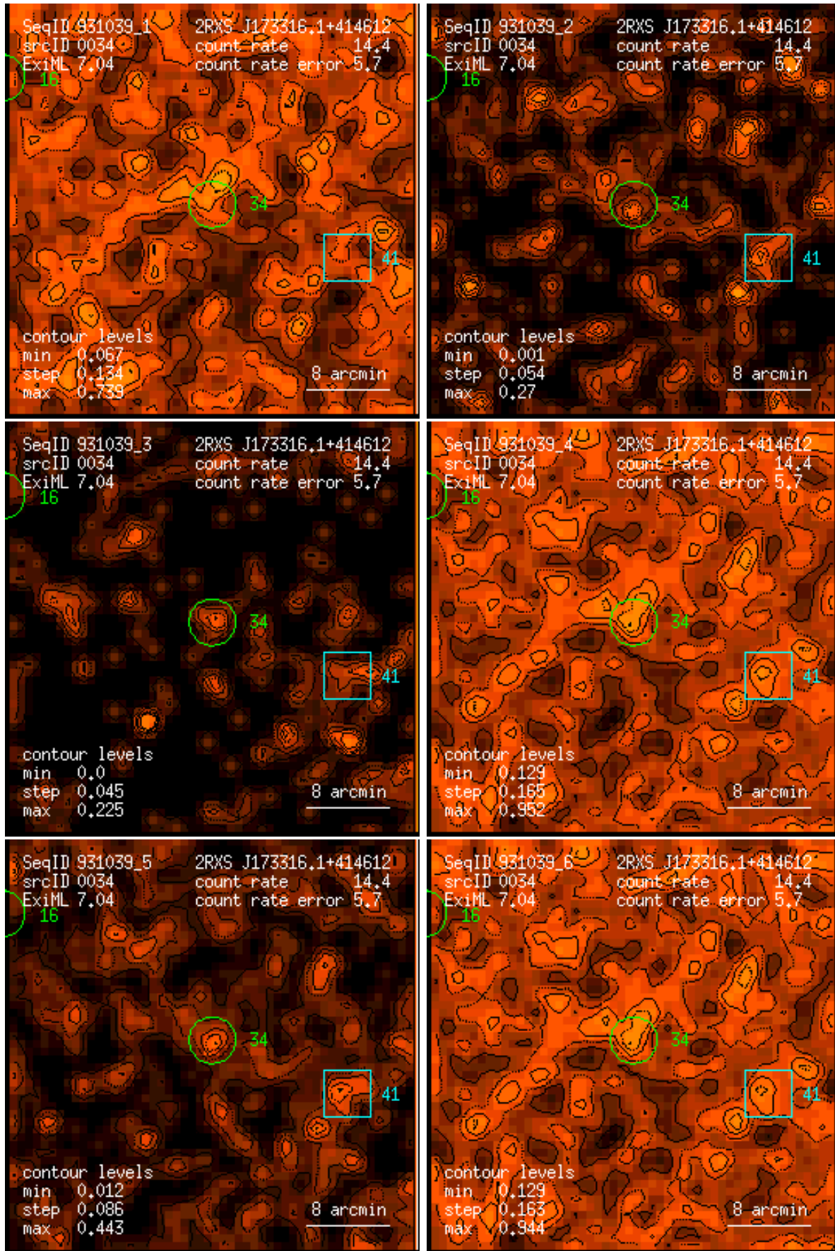
Figure 34: RASS 931039: detection 0034: band rate images, Gaussian filter: (1) PSPC channels 11 – 41, (2) 52 – 90, (3) 91 – 201, (4) 11 – 235, (5) 52 – 201, (6) 11 – 201. Broad band rates in counts/ks. Band rate contour levels in counts/ks/arcmin 2 .
