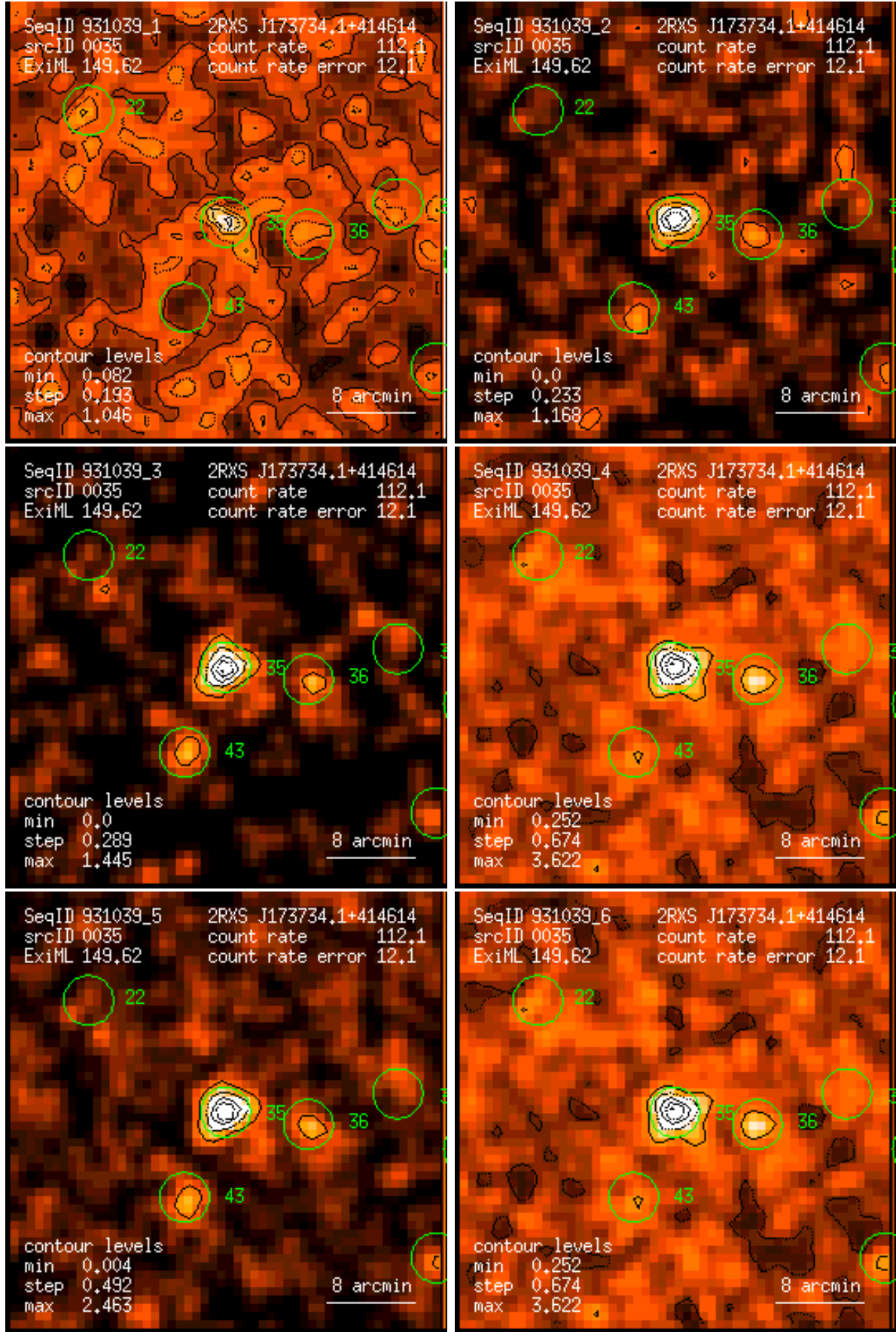
Figure 35: RASS 931039: detection 0035: band rate images, Gaussian filter: (1) PSPC channels 11 – 41, (2) 52 – 90, (3) 91 – 201, (4) 11 – 235, (5) 52 – 201, (6) 11 – 201. Broad band rates in counts/ks. Band rate contour levels in counts/ks/arcmin 2 .
