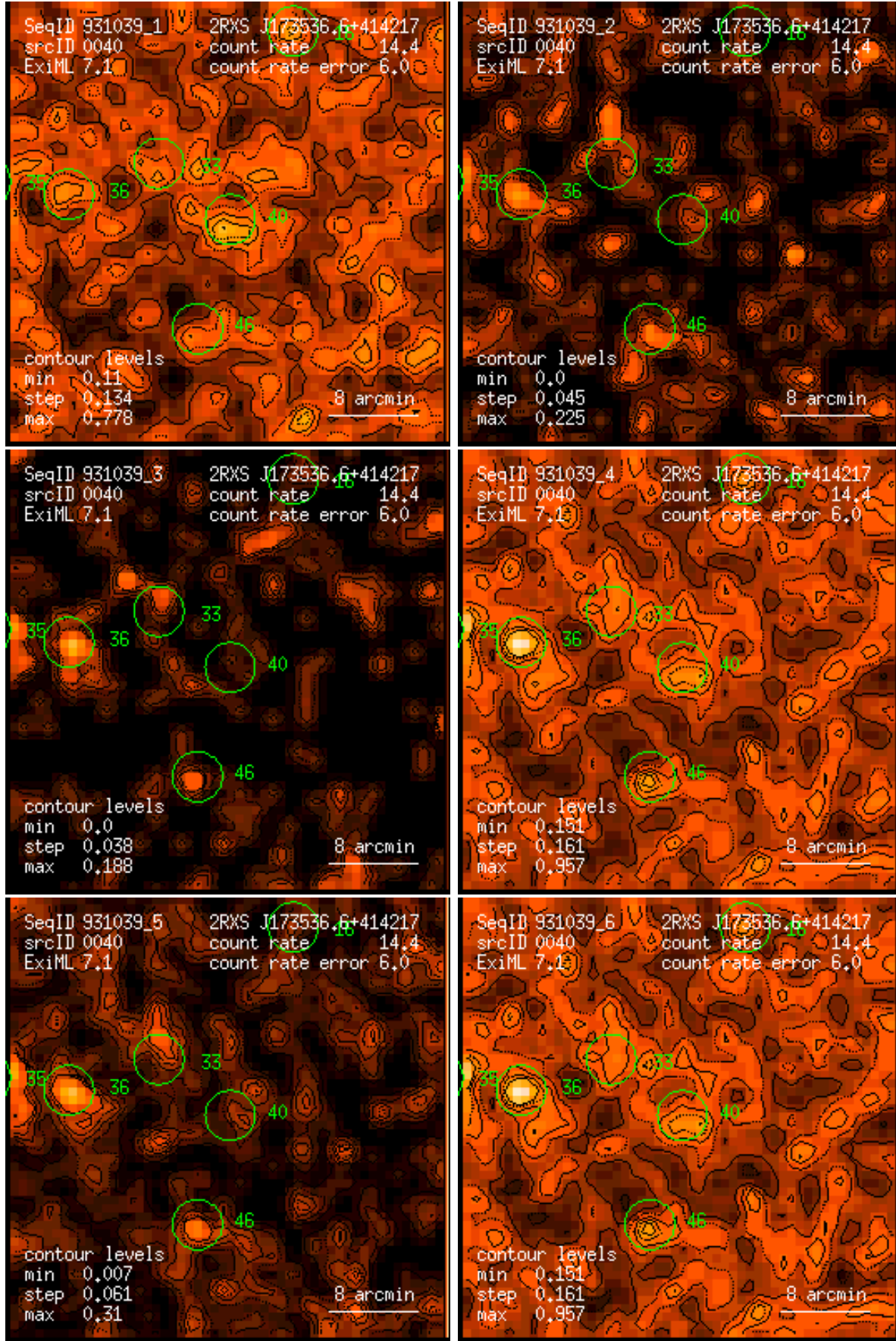
Figure 40: RASS 931039: detection 0040: band rate images, Gaussian filter: (1) PSPC channels 11 – 41, (2) 52 – 90, (3) 91 – 201, (4) 11 – 235, (5) 52 – 201, (6) 11 – 201. Broad band rates in counts/ks. Band rate contour levels in counts/ks/arcmin 2 .
