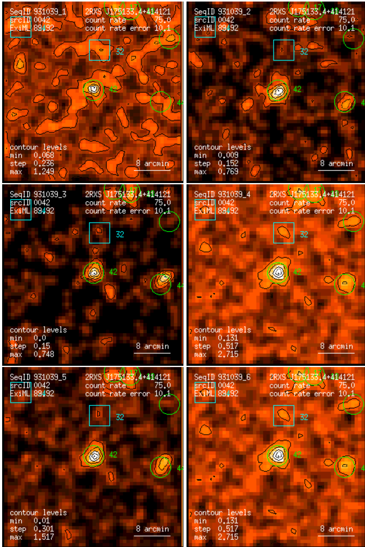
Figure 42: RASS 931039: detection 0042: band rate images, Gaussian filter: (1) PSPC channels 11 – 41, (2) 52 – 90, (3) 91 – 201, (4) 11 – 235, (5) 52 – 201, (6) 11 – 201. Broad band rates in counts/ks. Band rate contour levels in counts/ks/arcmin 2 .
