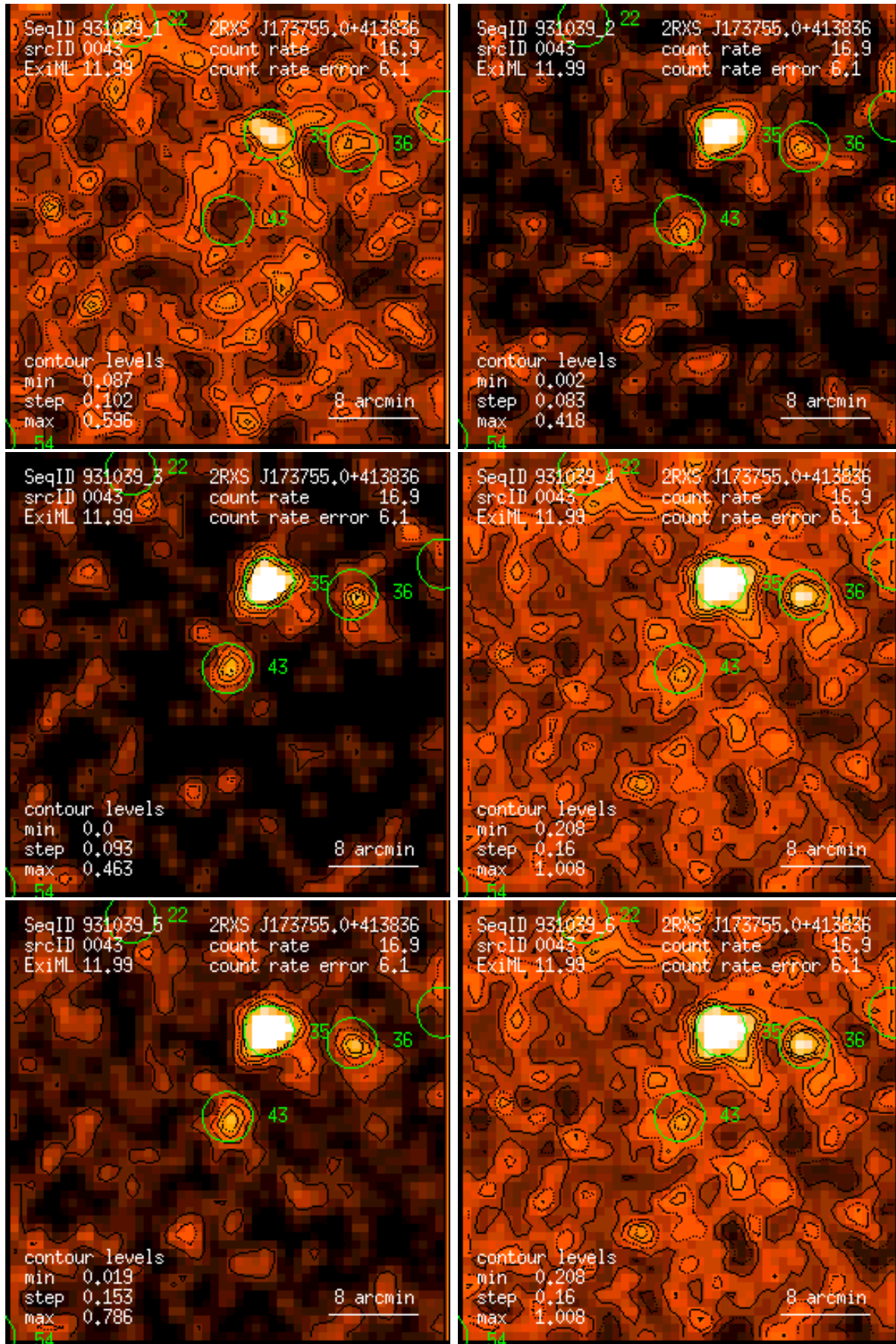
Figure 43: RASS 931039: detection 0043: band rate images, Gaussian filter: (1) PSPC channels 11 – 41, (2) 52 – 90, (3) 91 – 201, (4) 11 – 235, (5) 52 – 201, (6) 11 – 201. Broad band rates in counts/ks. Band rate contour levels in counts/ks/arcmin 2 .
