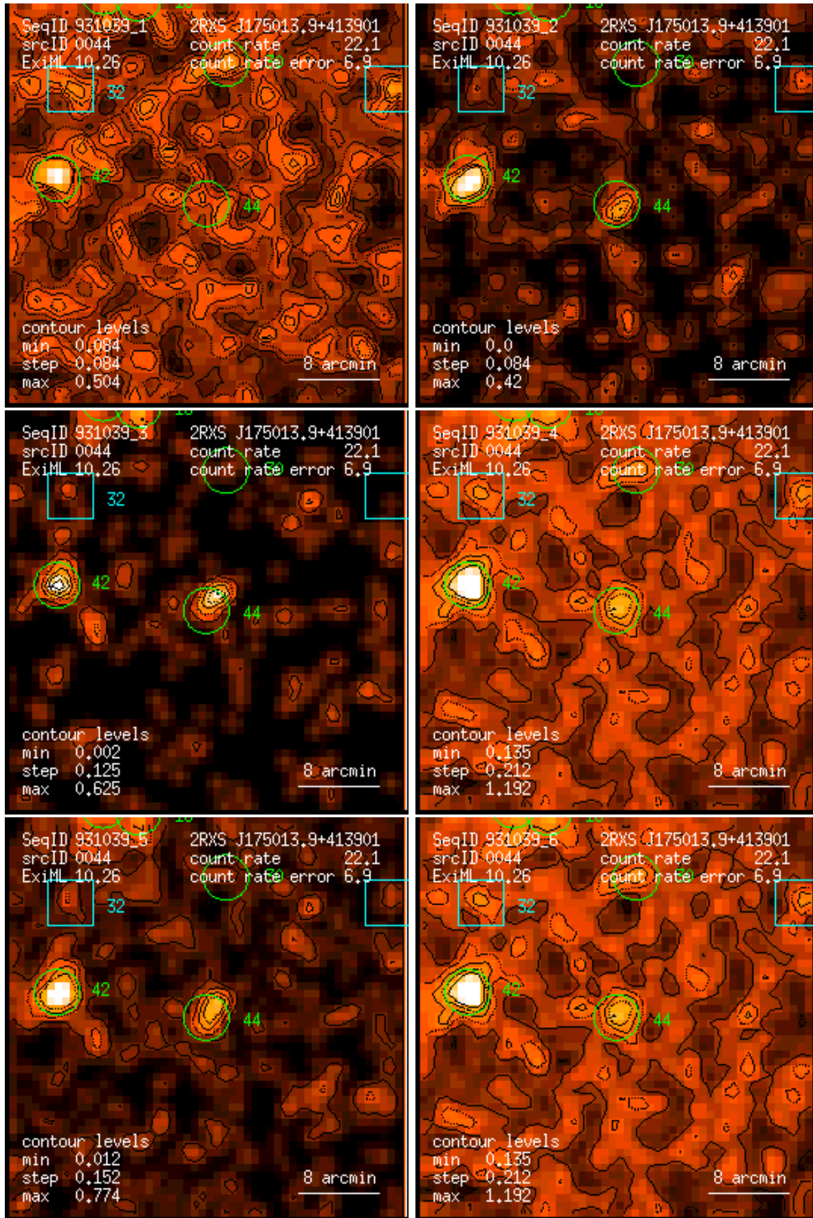
Figure 44: RASS 931039: detection 0044: band rate images, Gaussian filter: (1) PSPC channels 11 – 41, (2) 52 – 90, (3) 91 – 201, (4) 11 – 235, (5) 52 – 201, (6) 11 – 201. Broad band rates in counts/ks. Band rate contour levels in counts/ks/arcmin 2 .
