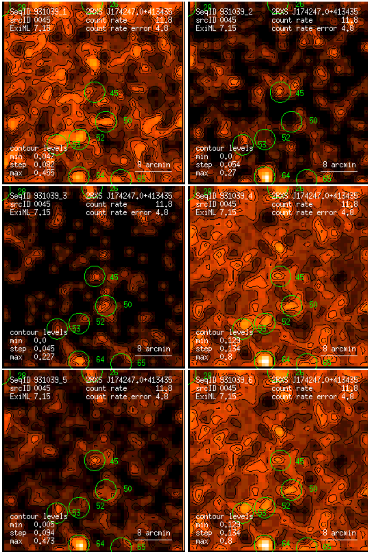
Figure 45: RASS 931039: detection 0045: band rate images, Gaussian filter: (1) PSPC channels 11 – 41, (2) 52 – 90, (3) 91 – 201, (4) 11 – 235, (5) 52 – 201, (6) 11 – 201. Broad band rates in counts/ks. Band rate contour levels in counts/ks/arcmin 2 .
