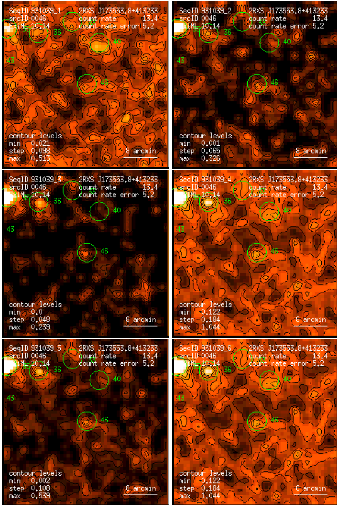
Figure 46: RASS 931039: detection 0046: band rate images, Gaussian filter: (1) PSPC channels 11 – 41, (2) 52 – 90, (3) 91 – 201, (4) 11 – 235, (5) 52 – 201, (6) 11 – 201. Broad band rates in counts/ks. Band rate contour levels in counts/ks/arcmin 2 .
