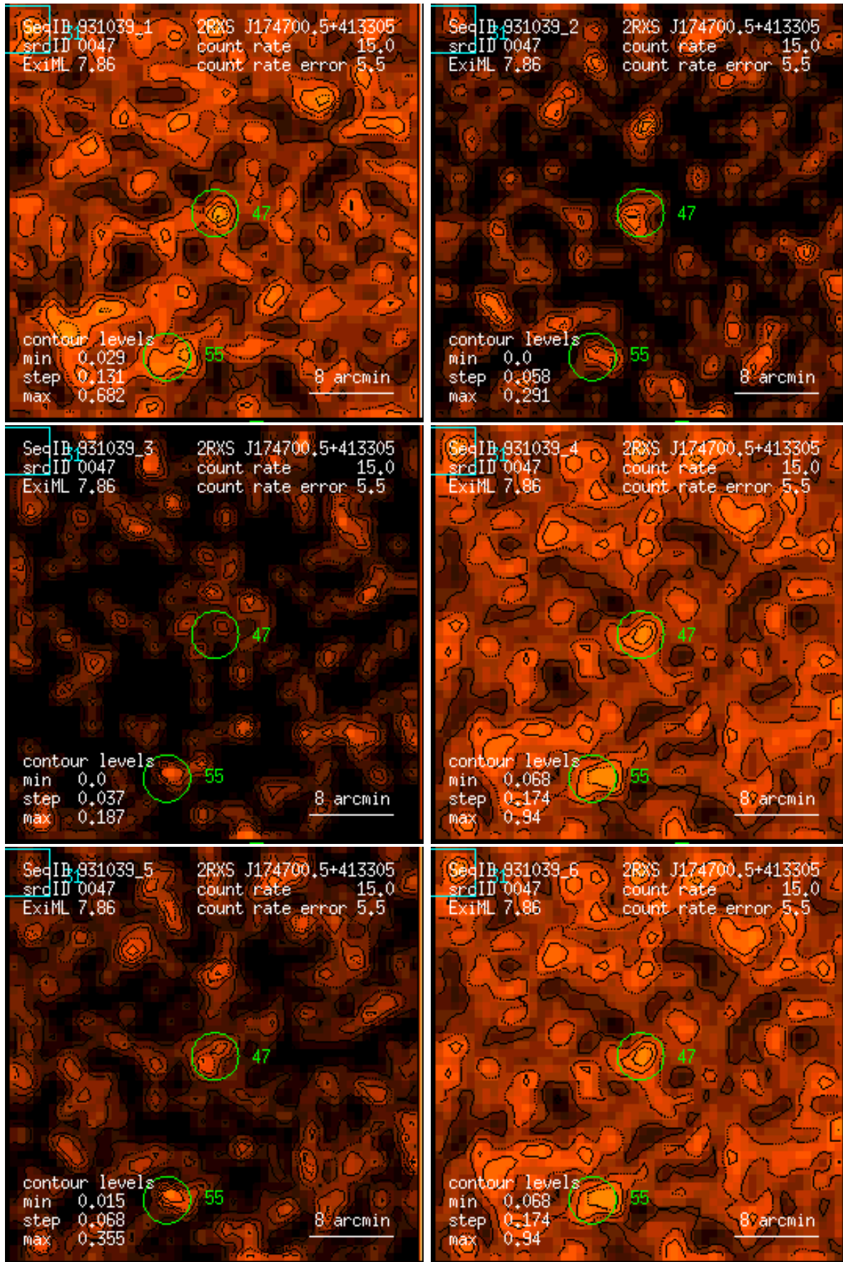
Figure 47: RASS 931039: detection 0047: band rate images, Gaussian filter: (1) PSPC channels 11 – 41, (2) 52 – 90, (3) 91 – 201, (4) 11 – 235, (5) 52 – 201, (6) 11 – 201. Broad band rates in counts/ks. Band rate contour levels in counts/ks/arcmin 2 .
