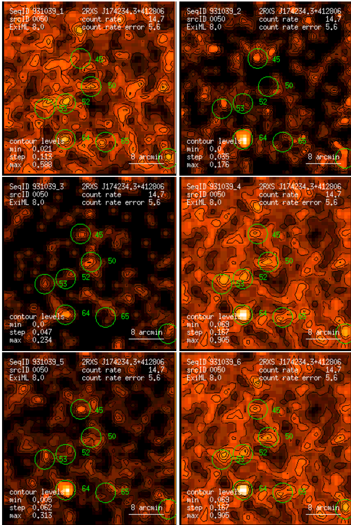
Figure 50: RASS 931039: detection 0050: band rate images, Gaussian filter: (1) PSPC channels 11 – 41, (2) 52 – 90, (3) 91 – 201, (4) 11 – 235, (5) 52 – 201, (6) 11 – 201. Broad band rates in counts/ks. Band rate contour levels in counts/ks/arcmin 2 .
