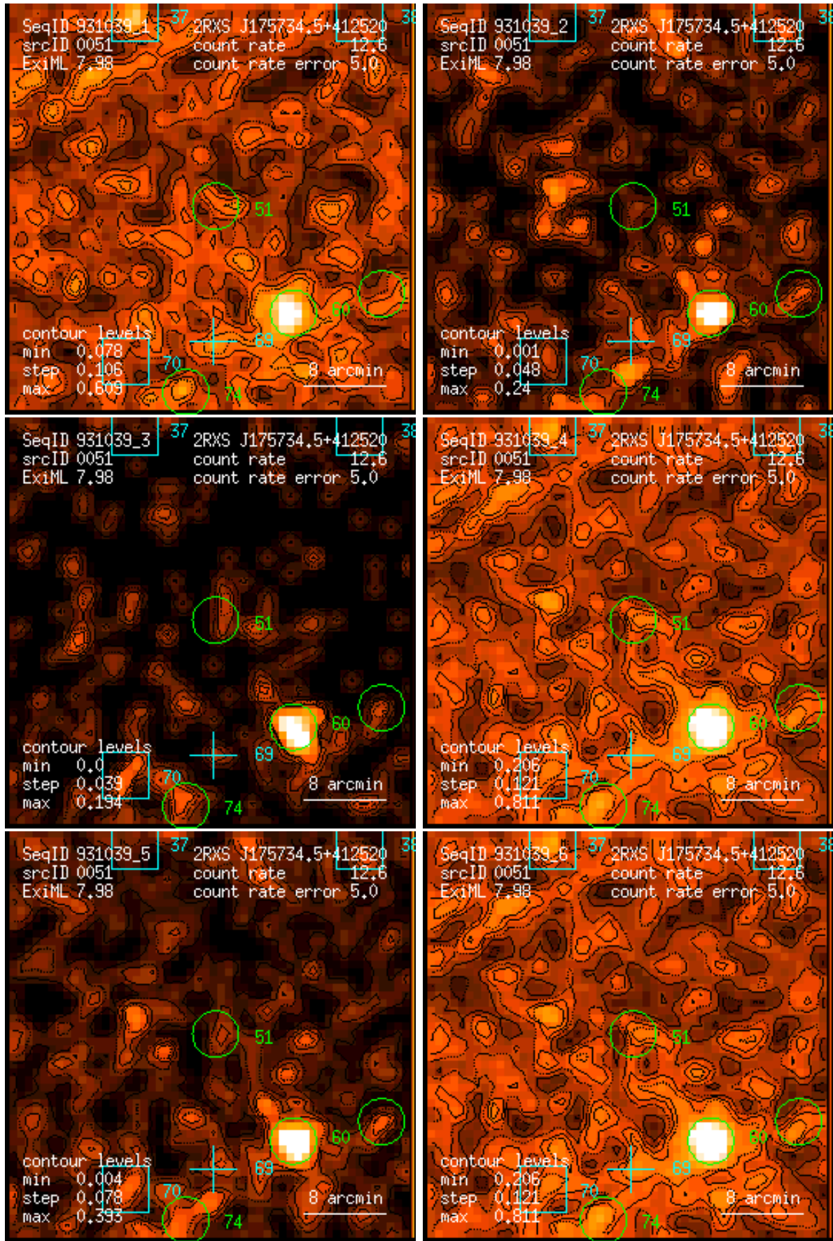
Figure 51: RASS 931039: detection 0051: band rate images, Gaussian filter: (1) PSPC channels 11 – 41, (2) 52 – 90, (3) 91 – 201, (4) 11 – 235, (5) 52 – 201, (6) 11 – 201. Broad band rates in counts/ks. Band rate contour levels in counts/ks/arcmin 2 .
