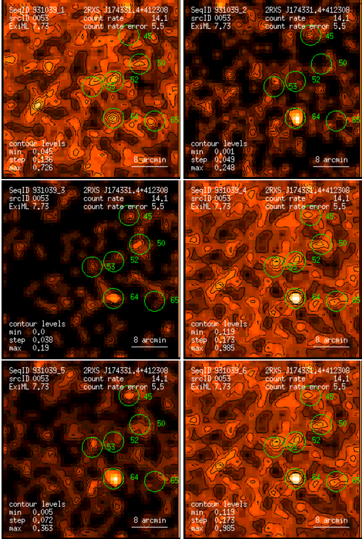
Figure 53: RASS 931039: detection 0053: band rate images, Gaussian filter: (1) PSPC channels 11 – 41, (2) 52 – 90, (3) 91 – 201, (4) 11 – 235, (5) 52 – 201, (6) 11 – 201. Broad band rates in counts/ks. Band rate contour levels in counts/ks/arcmin 2 .
