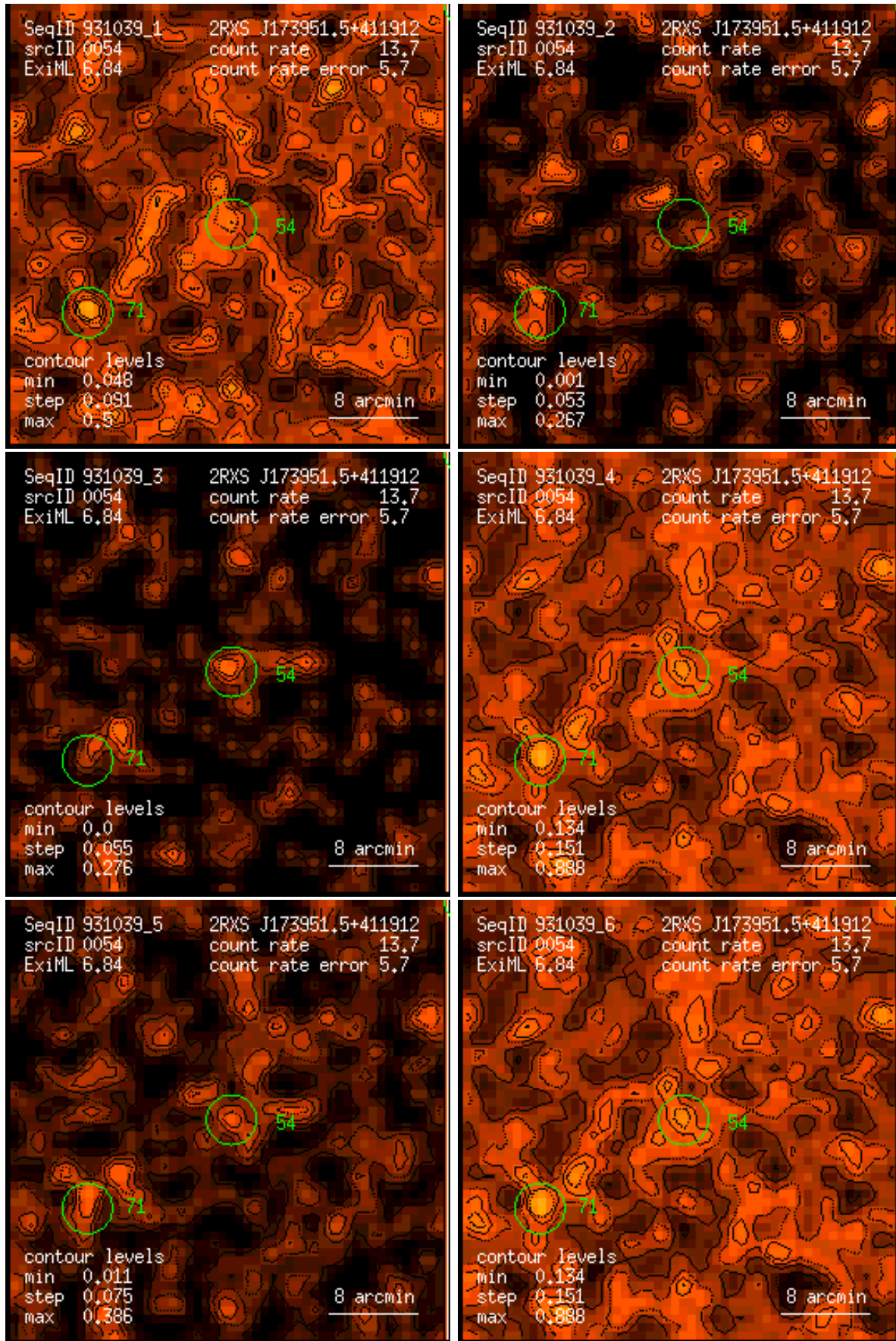
Figure 54: RASS 931039: detection 0054: band rate images, Gaussian filter: (1) PSPC channels 11 – 41, (2) 52 – 90, (3) 91 – 201, (4) 11 – 235, (5) 52 – 201, (6) 11 – 201. Broad band rates in counts/ks. Band rate contour levels in counts/ks/arcmin 2 .
