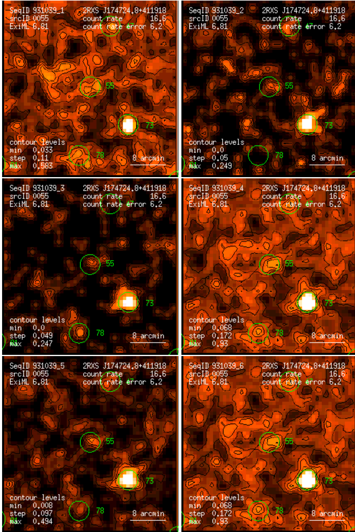
Figure 55: RASS 931039: detection 0055: band rate images, Gaussian filter: (1) PSPC channels 11 – 41, (2) 52 – 90, (3) 91 – 201, (4) 11 – 235, (5) 52 – 201, (6) 11 – 201. Broad band rates in counts/ks. Band rate contour levels in counts/ks/arcmin 2 .
