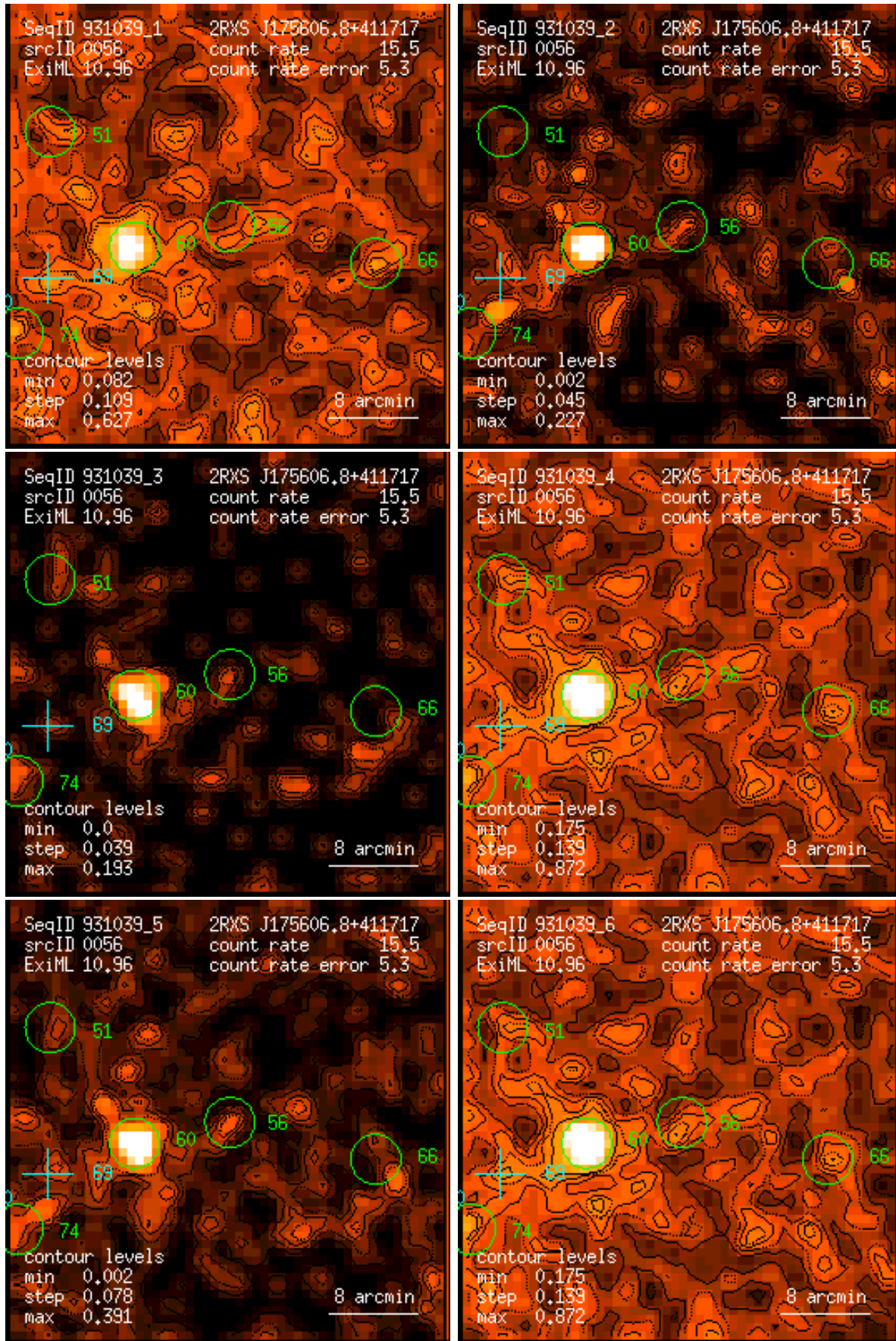
Figure 56: RASS 931039: detection 0056: band rate images, Gaussian filter: (1) PSPC channels 11 – 41, (2) 52 – 90, (3) 91 – 201, (4) 11 – 235, (5) 52 – 201, (6) 11 – 201. Broad band rates in counts/ks. Band rate contour levels in counts/ks/arcmin 2 .
