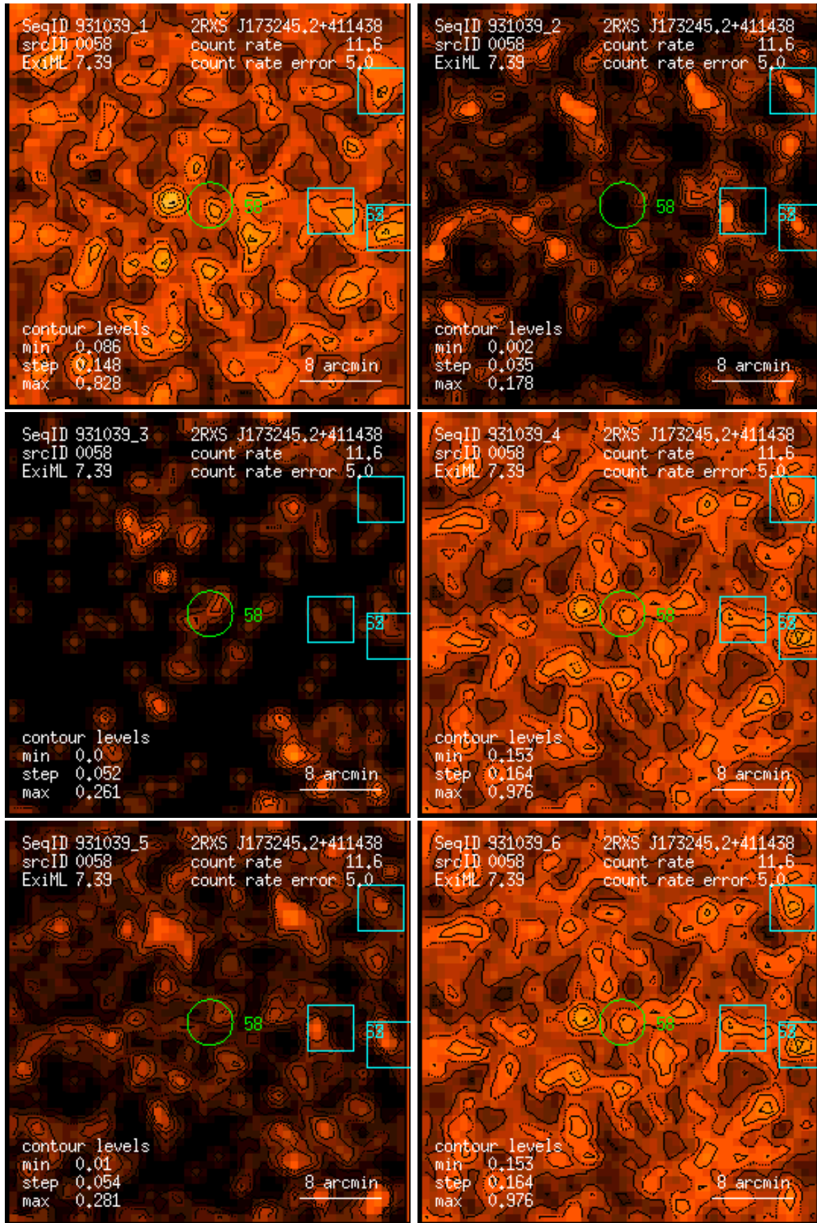
Figure 58: RASS 931039: detection 0058: band rate images, Gaussian filter: (1) PSPC channels 11 – 41, (2) 52 – 90, (3) 91 – 201, (4) 11 – 235, (5) 52 – 201, (6) 11 – 201. Broad band rates in counts/ks. Band rate contour levels in counts/ks/arcmin 2 .
