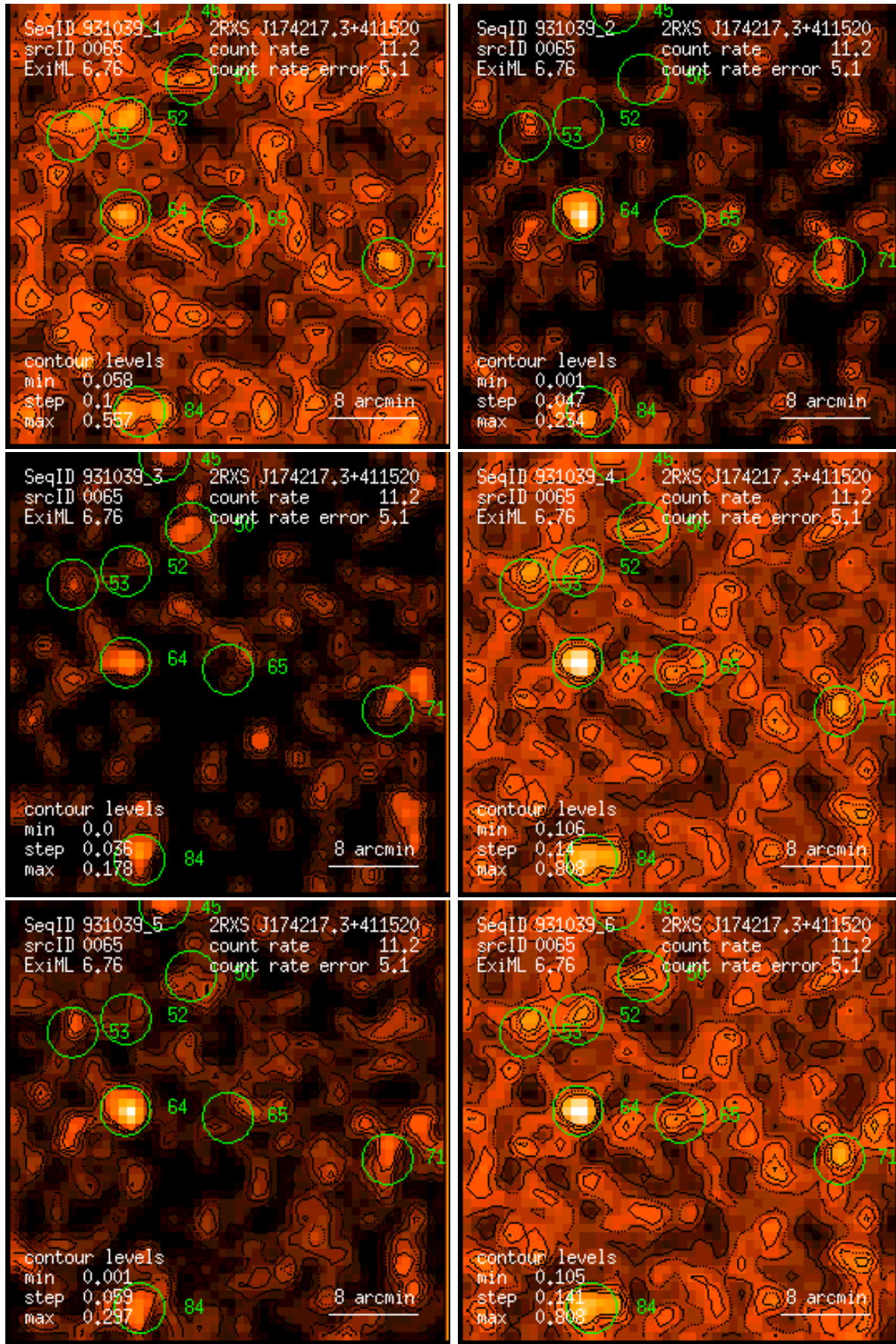
Figure 65: RASS 931039: detection 0065: band rate images, Gaussian filter: (1) PSPC channels 11 – 41, (2) 52 – 90, (3) 91 – 201, (4) 11 – 235, (5) 52 – 201, (6) 11 – 201. Broad band rates in counts/ks. Band rate contour levels in counts/ks/arcmin 2 .
