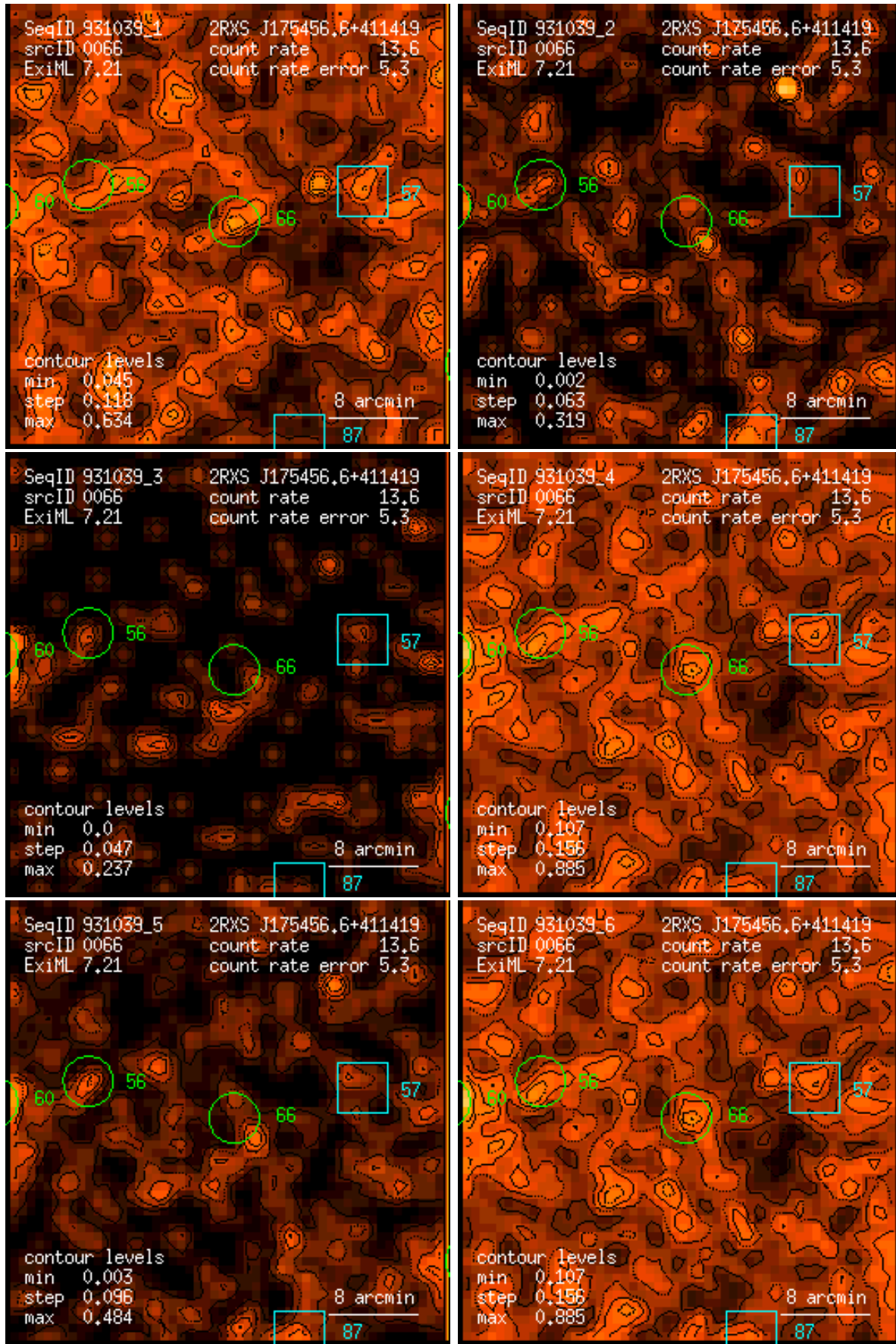
Figure 66: RASS 931039: detection 0066: band rate images, Gaussian filter: (1) PSPC channels 11 – 41, (2) 52 – 90, (3) 91 – 201, (4) 11 – 235, (5) 52 – 201, (6) 11 – 201. Broad band rates in counts/ks. Band rate contour levels in counts/ks/arcmin 2 .
