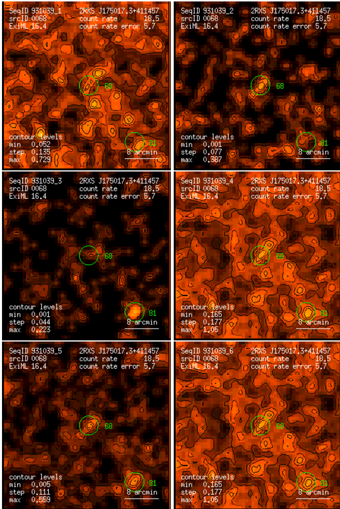
Figure 68: RASS 931039: detection 0068: band rate images, Gaussian filter: (1) PSPC channels 11 – 41, (2) 52 – 90, (3) 91 – 201, (4) 11 – 235, (5) 52 – 201, (6) 11 – 201. Broad band rates in counts/ks. Band rate contour levels in counts/ks/arcmin 2 .
