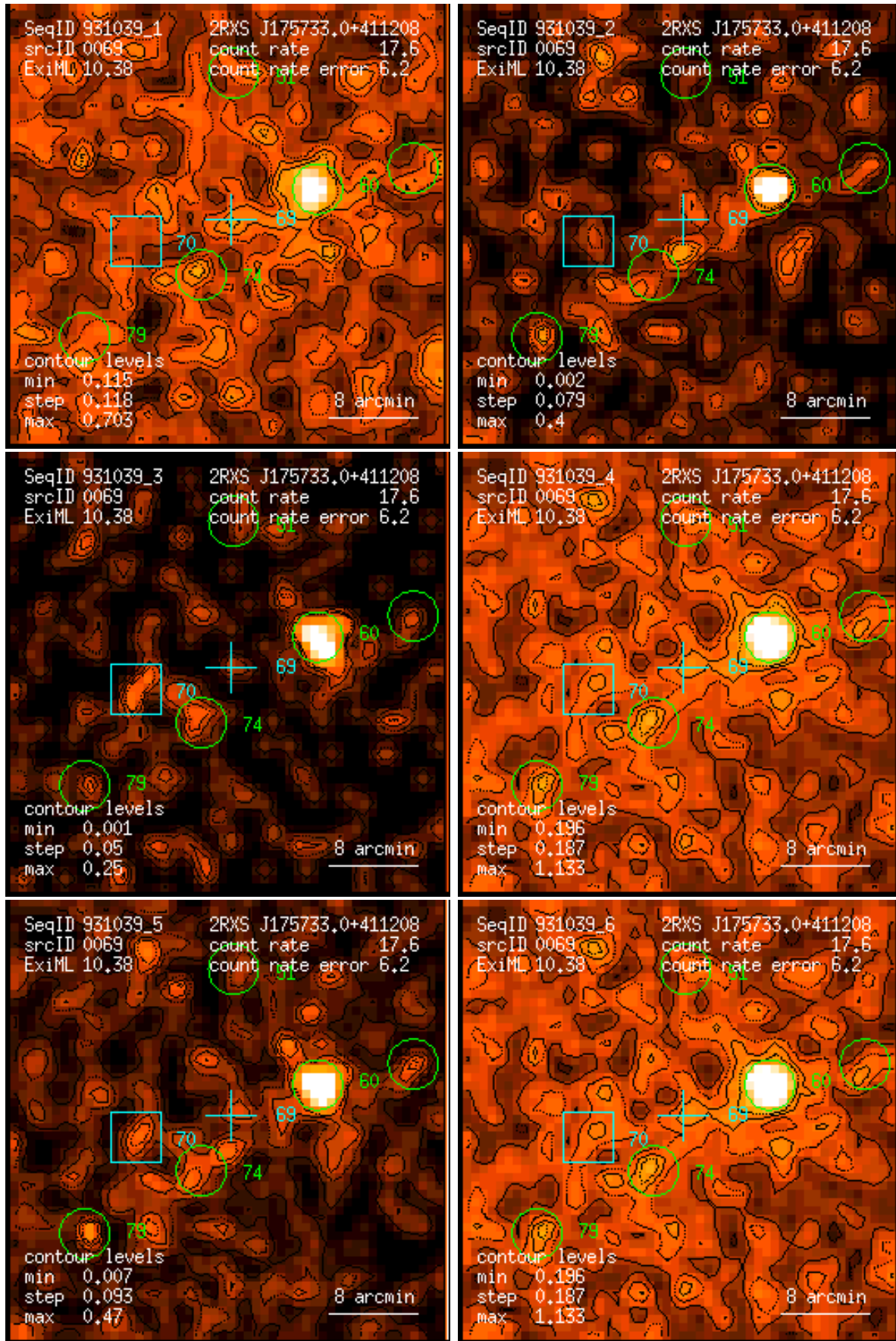
Figure 69: RASS 931039: detection 0069: band rate images, Gaussian filter: (1) PSPC channels 11 – 41, (2) 52 – 90, (3) 91 – 201, (4) 11 – 235, (5) 52 – 201, (6) 11 – 201. Broad band rates in counts/ks. Band rate contour levels in counts/ks/arcmin 2 .
